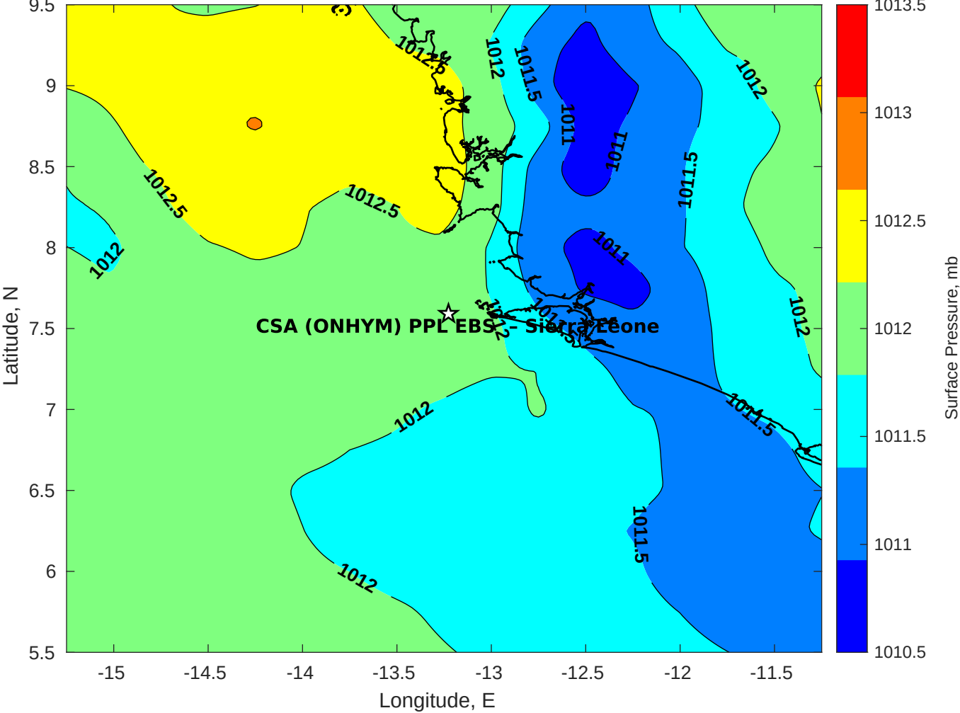
Surface Pressure (mb) for CSA (ONHYM) PPL EBS - Sierra Leone at 19-Apr-2025 00:00:00
