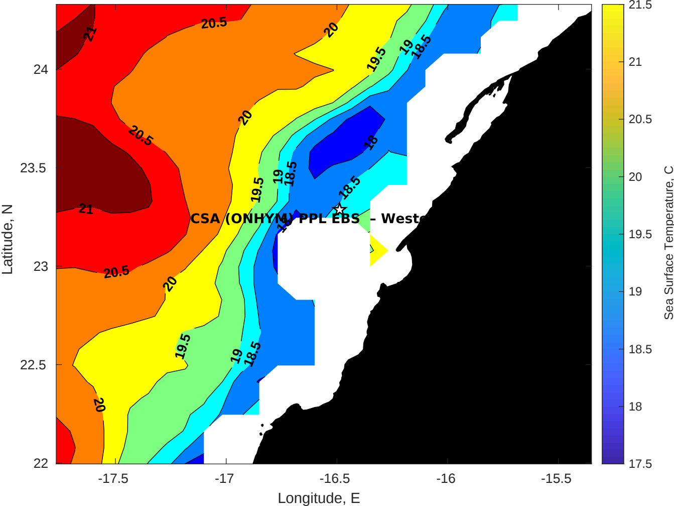
SST for CSA (ONHYM) PPL EBS - Western Sahara at 17-Apr-2025 00:00:00
