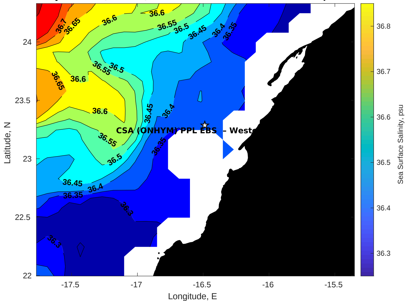
Surface Salinity for CSA (ONHYM) PPL EBS - Western Sahara at 17-Apr-2025 00:00:00
