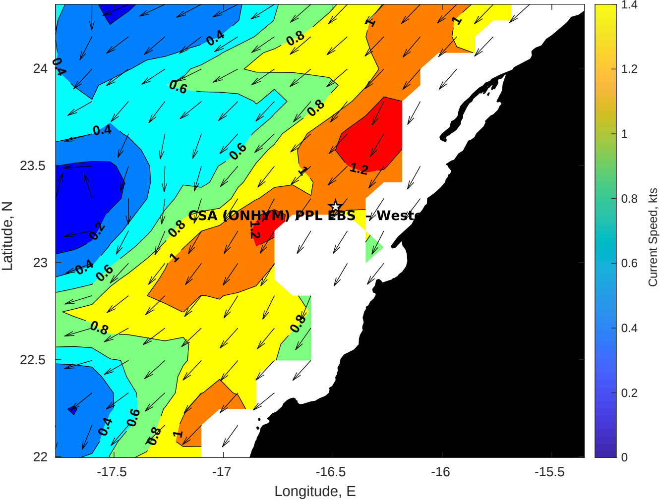
Surface Currents for CSA (ONHYM) PPL EBS - Western Sahara at 17-Apr-2025 00:00:00
