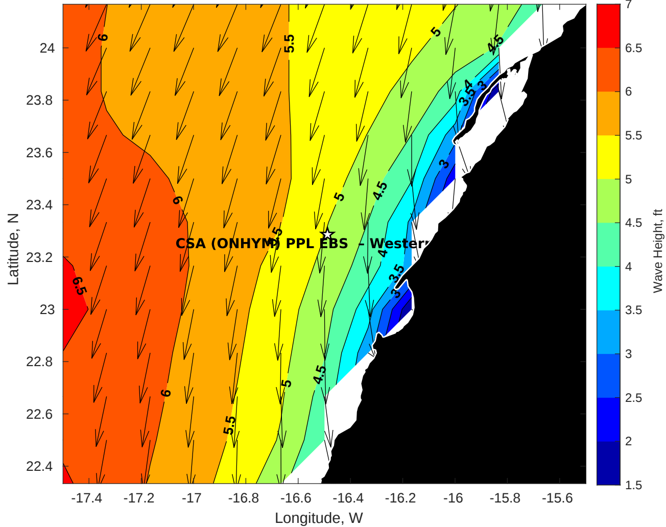
Wave Height (ft) for CSA (ONHYM) PPL EBS - Western Sahara at 18-Apr-2025 09:00:00
