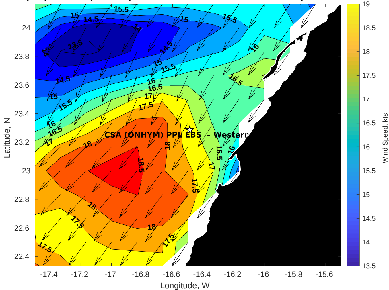
Winds (kts) for CSA (ONHYM) PPL EBS - Western Sahara at 18-Apr-2025 09:00:00
