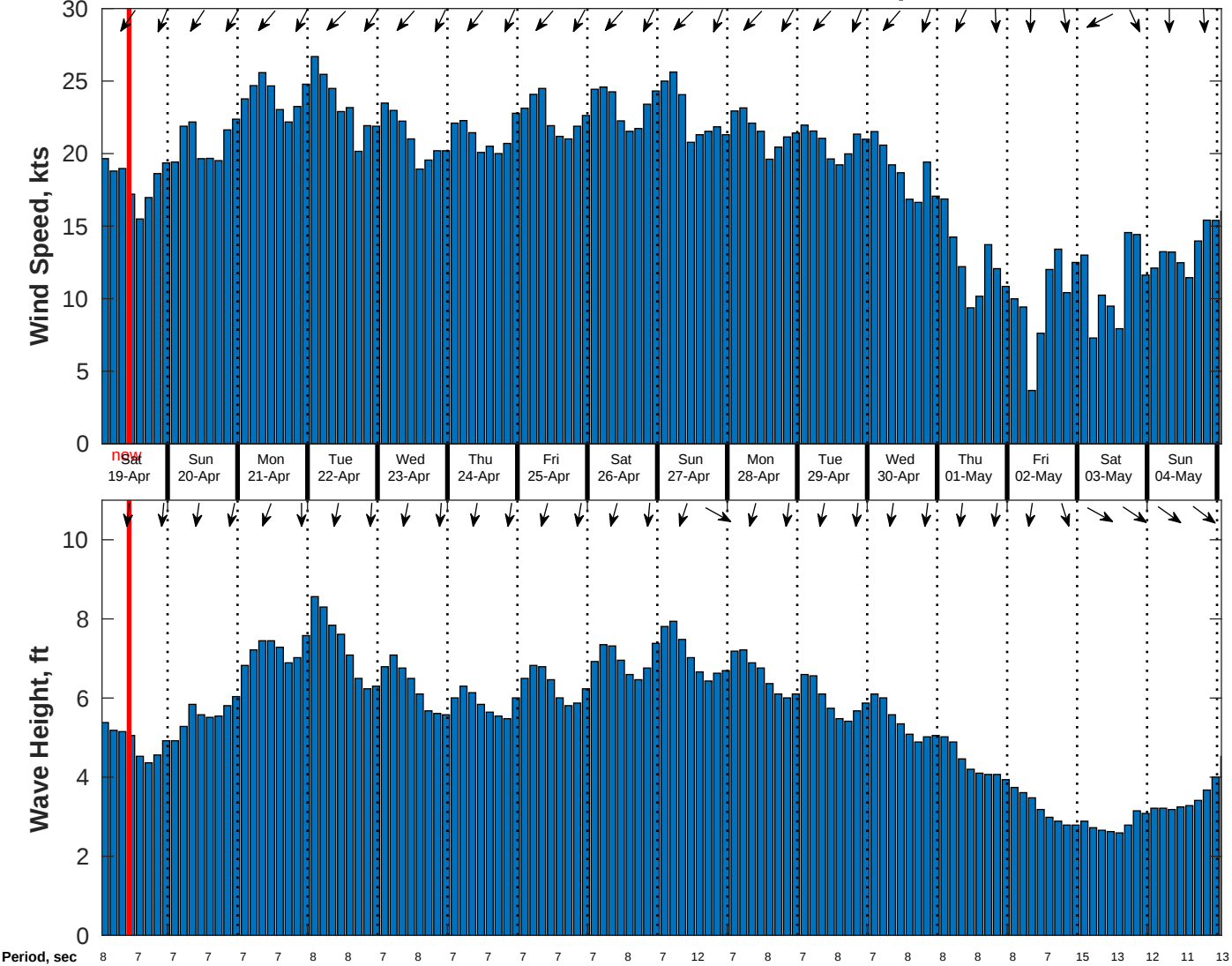
Wind & Wave Forecast for CSA (ONHYM) PPL EBS - Western Sahara from 18-Apr-2025 01:00:00 to 04-May-2025 01:00:00
