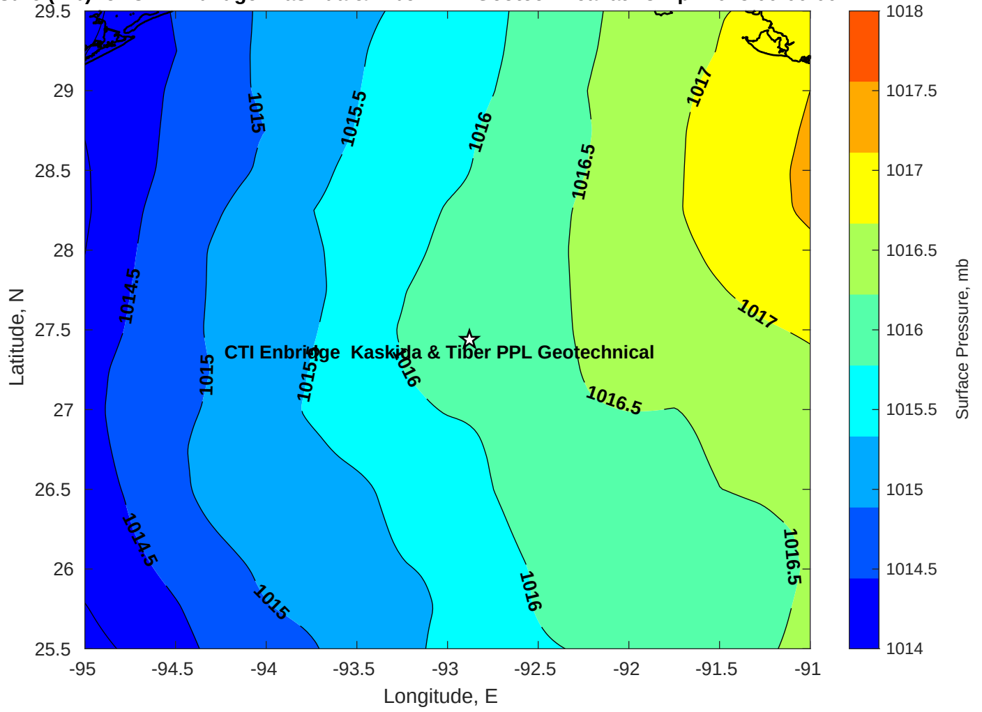
Surface Pressure (mb) for CTI Enbridge Kaskida & Tiber PPL Geotechnical at 18-Apr-2025 00:00:00
