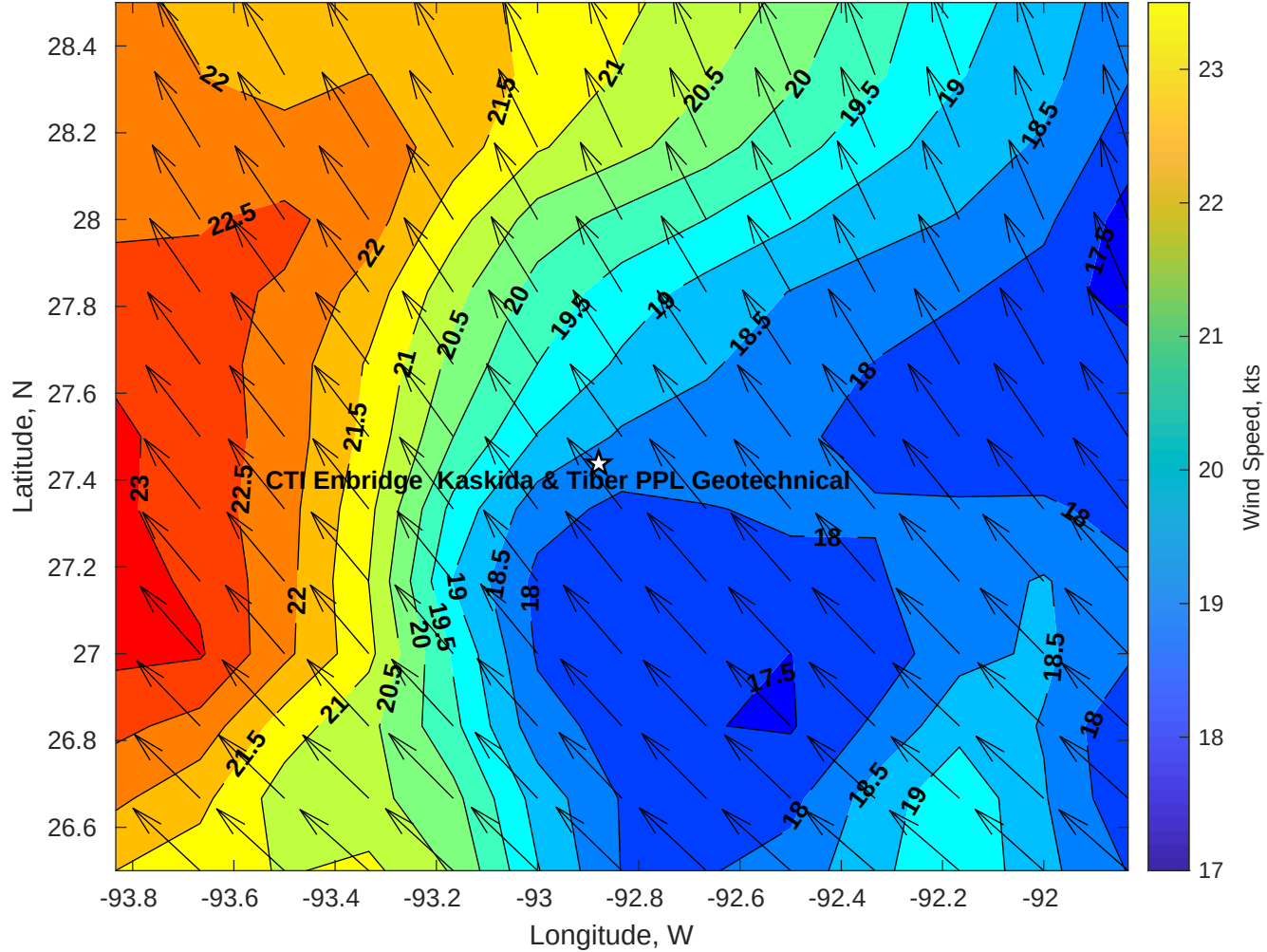
Winds (kts) for CTI Enbridge Kaskida & Tiber PPL Geotechnical at 18-Apr-2025 09:00:00
