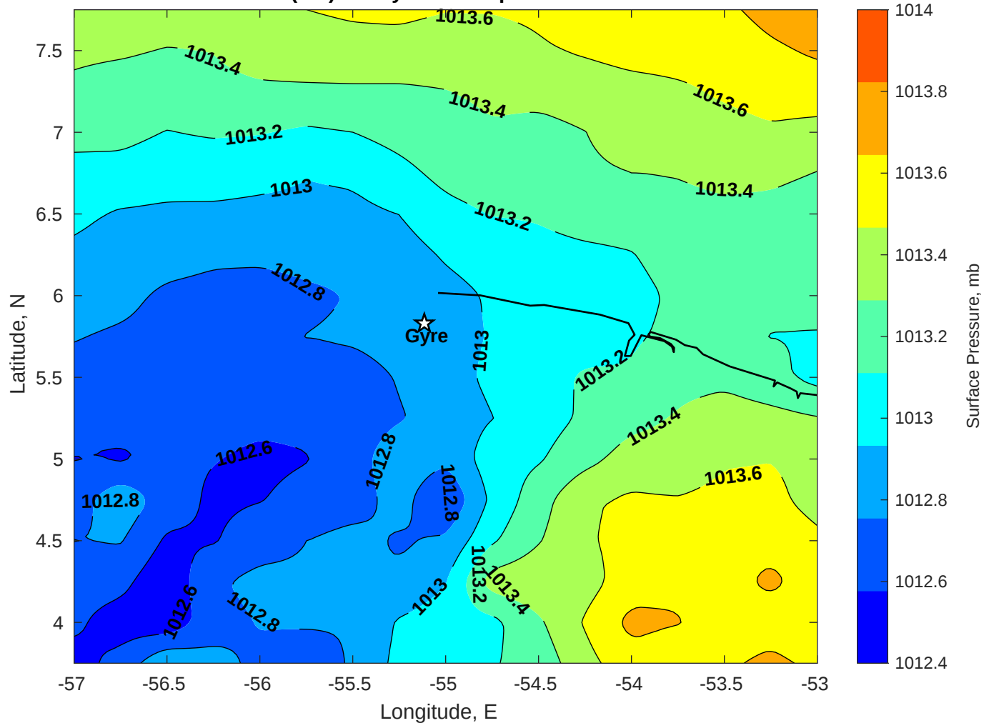
Surface Pressure (mb) for Gyre at 19-Apr-2025 00:00:00
