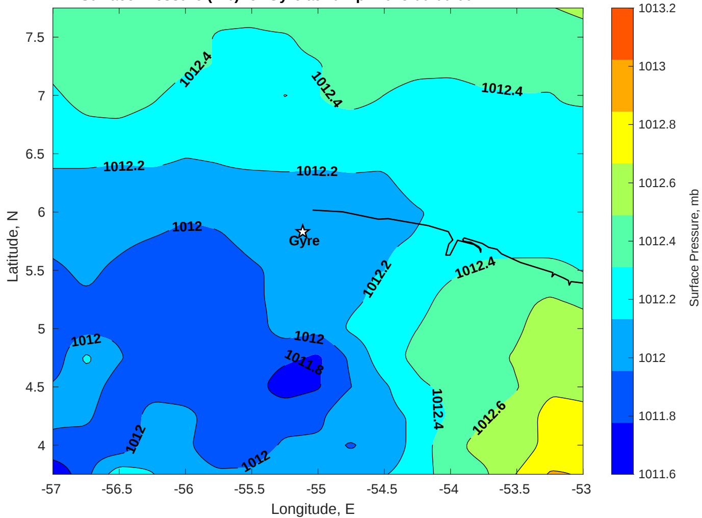
Surface Pressure (mb) for Gyre at 20-Apr-2025 00:00:00
