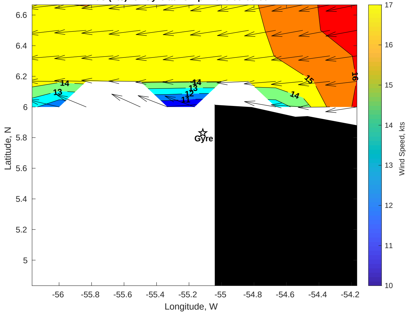
Winds (kts) for Gyre at 18-Apr-2025 09:00:00
