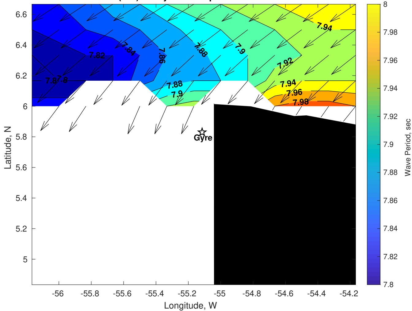
Wave Period (sec) for Gyre at 18-Apr-2025 09:00:00
