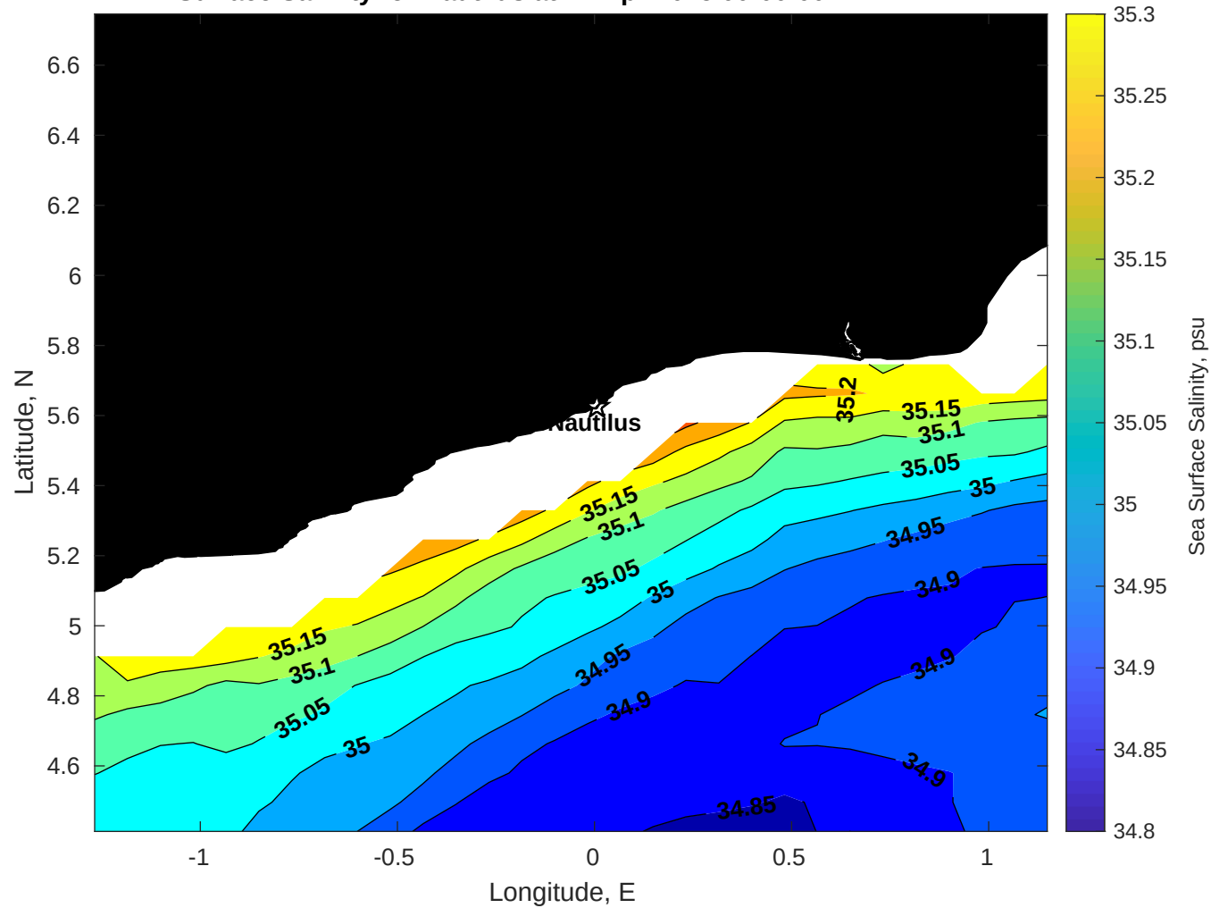
Surface Salinity for Nautilus at 17-Apr-2025 00:00:00
