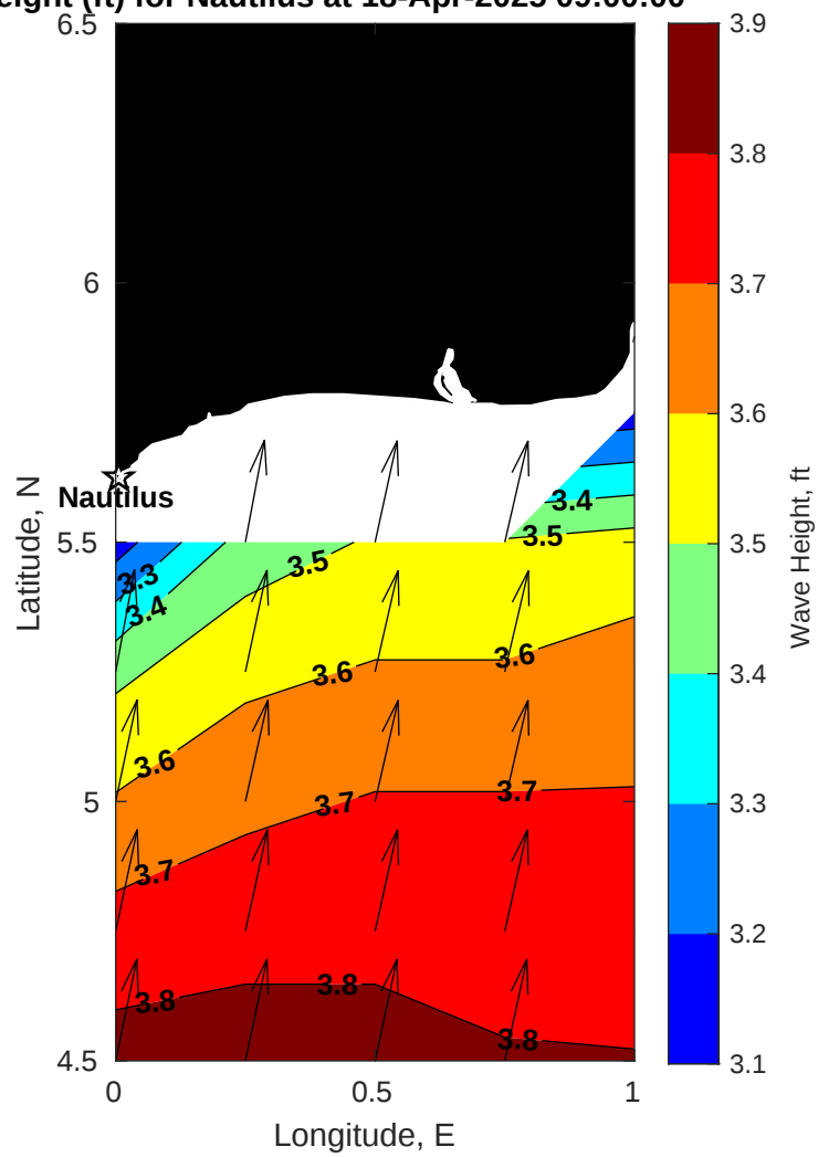
Wave Height (ft) for Nautilus at 18-Apr-2025 09:00:00
