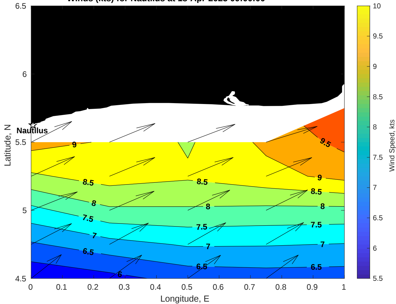
Winds (kts) for Nautilus at 18-Apr-2025 09:00:00
