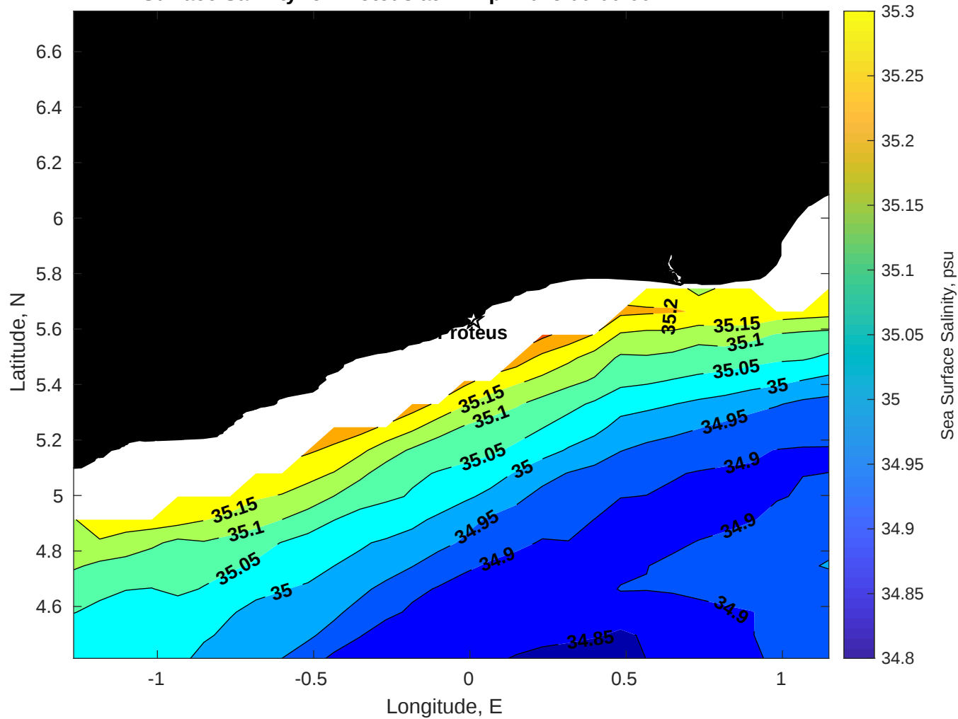
Surface Salinity for Proteus at 17-Apr-2025 00:00:00
