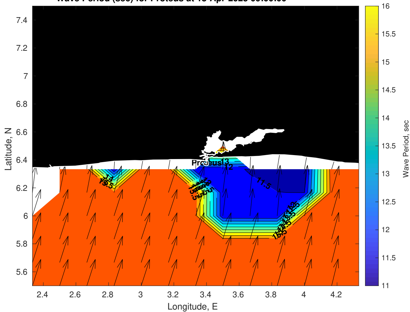
Wave Period (sec) for Proteus at 18-Apr-2025 09:00:00
