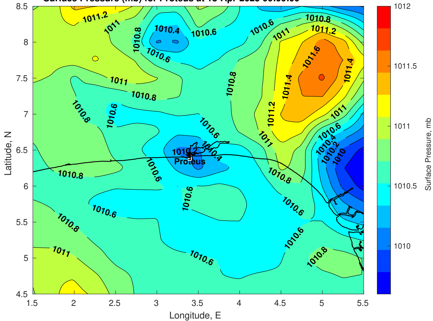
Surface Pressure (mb) for Proteus at 18-Apr-2025 00:00:00
