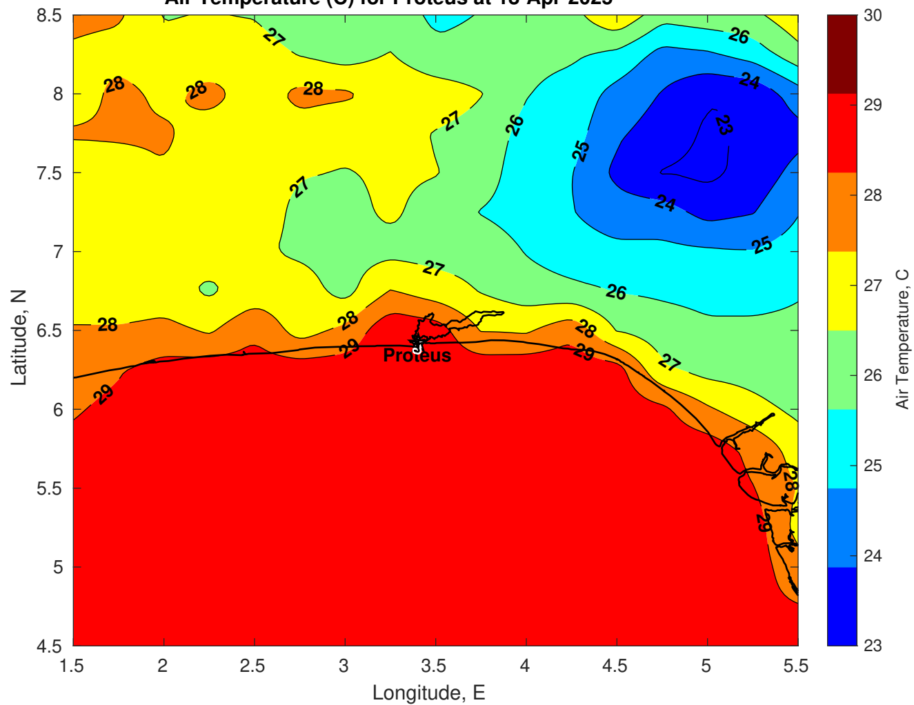
Air Temperature (C) for Proteus at 18-Apr-2025
