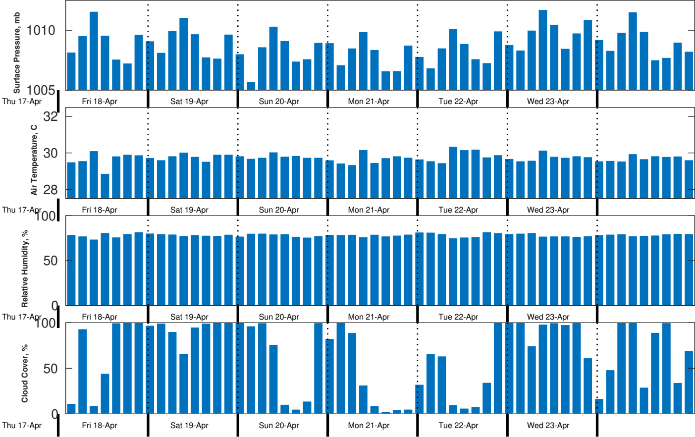
Met Forecast for Proteus from 18-Apr-2025 00:00:00 to 25-Apr-2025 00:00:00
