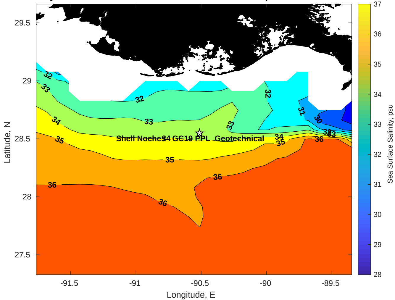
Surface Salinity for Shell Noches GC19 PPL Geotechnical at 17-Apr-2025 00:00:00
