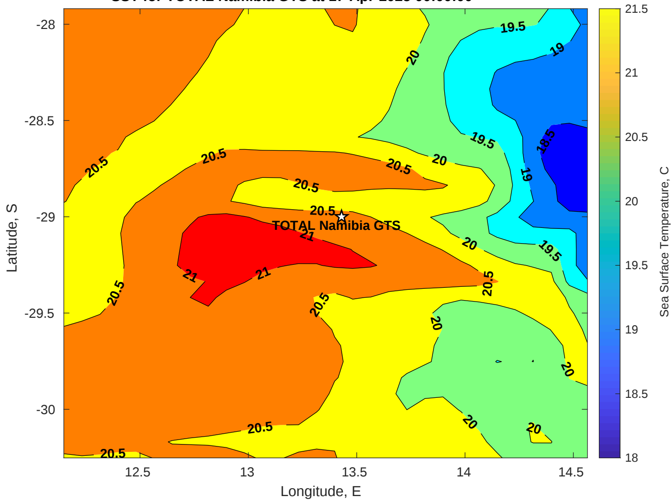
SST for TOTAL Namibia GTS at 17-Apr-2025 00:00:00
