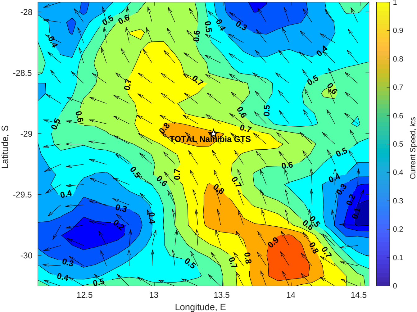
Surface Currents for TOTAL Namibia GTS at 17-Apr-2025 00:00:00
