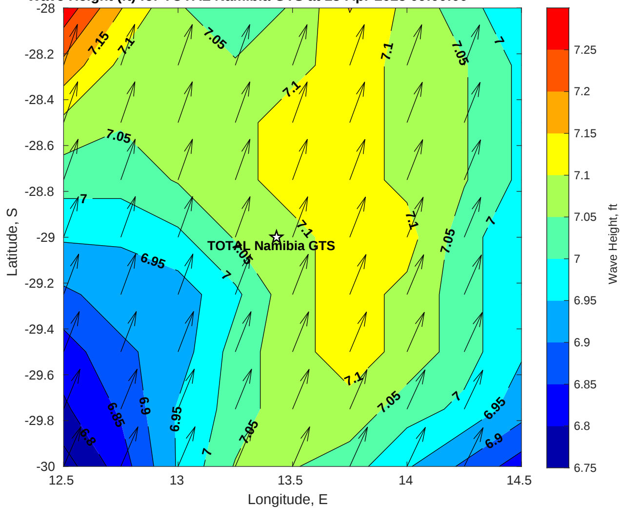
Wave Height (ft) for TOTAL Namibia GTS at 18-Apr-2025 09:00:00
