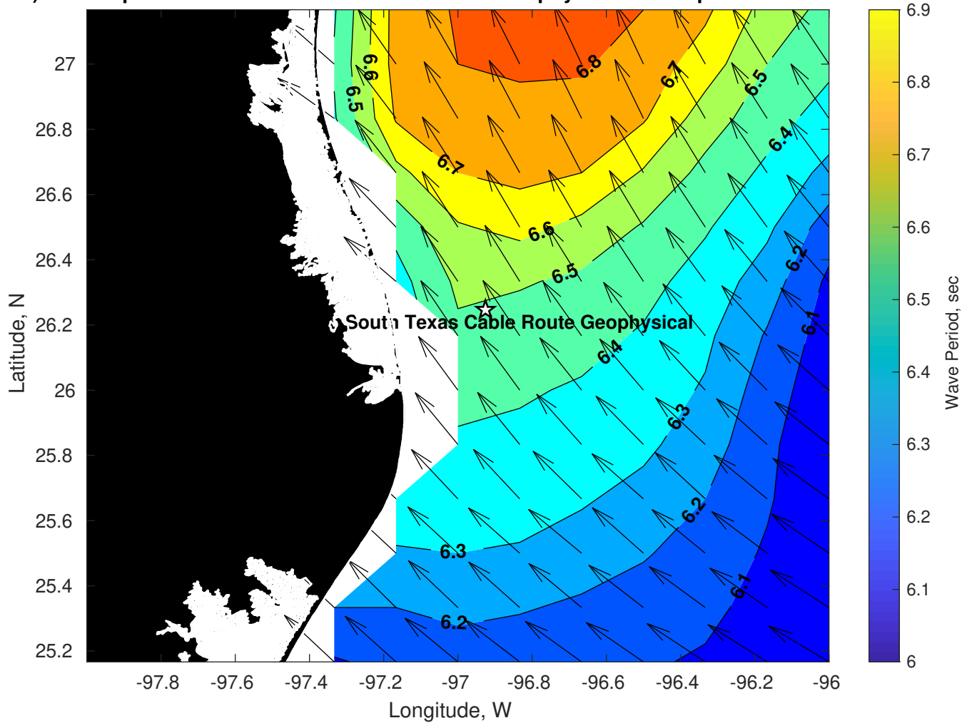
Period (sec) for Tampnet P2378 South Texas Cable Route Geophysical at 18-Apr-2025 09:00:00
