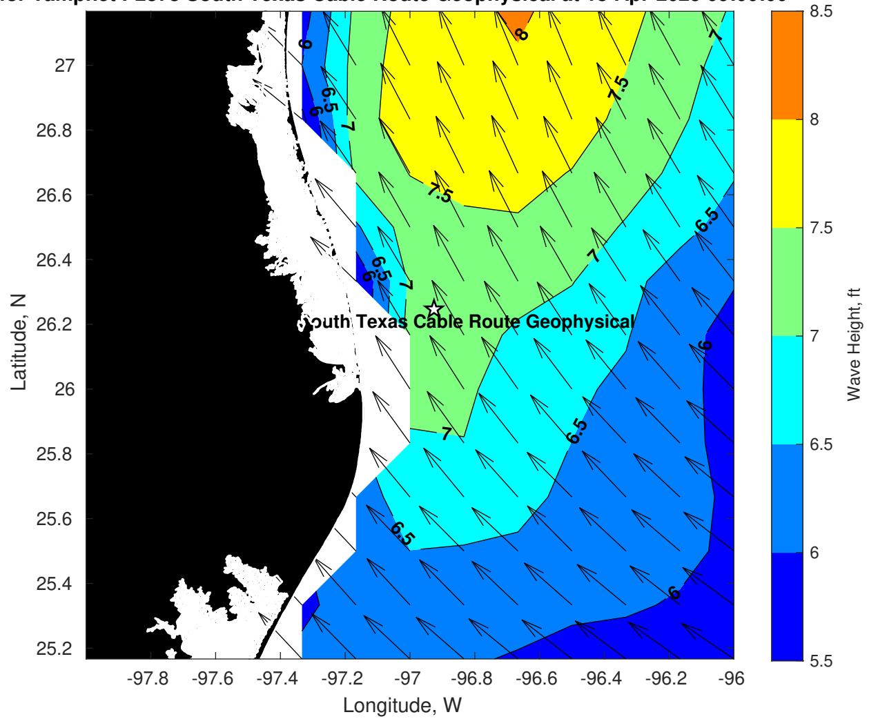
Wave Height (ft) for Tampnet P2378 South Texas Cable Route Geophysical at 18-Apr-2025 09:00:00
