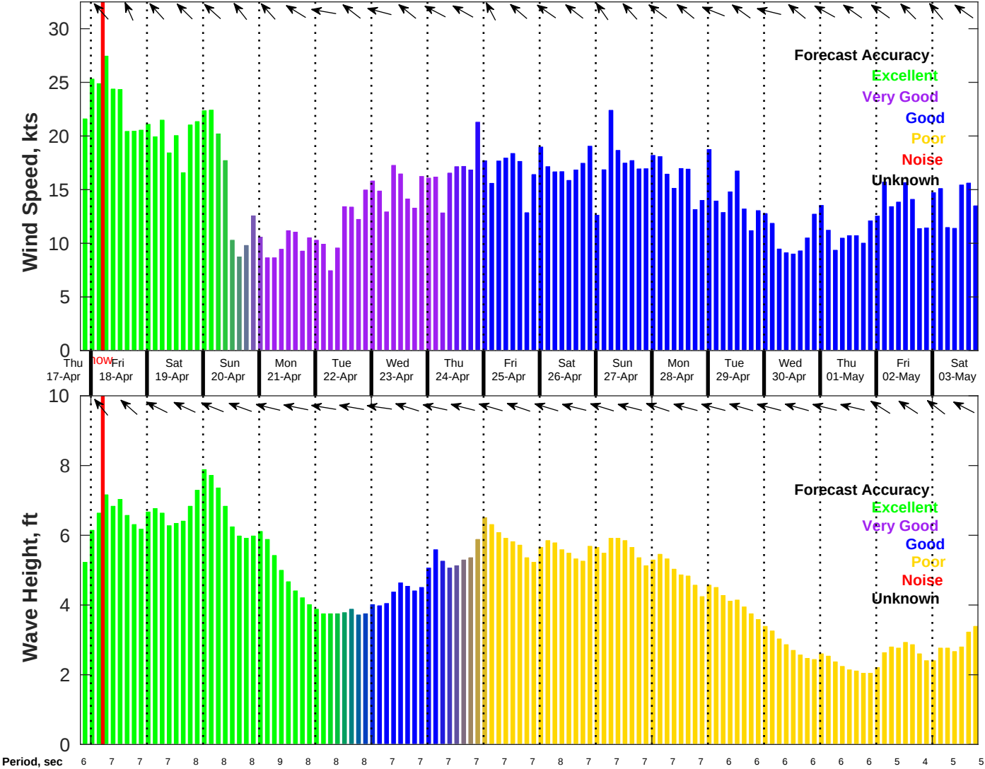
Wind & Wave Forecast for Tampnet P2378 South Texas Cable Route Geophysical from 17-Apr-2025 20:00:00 to 03-May-2025 20:00:00
