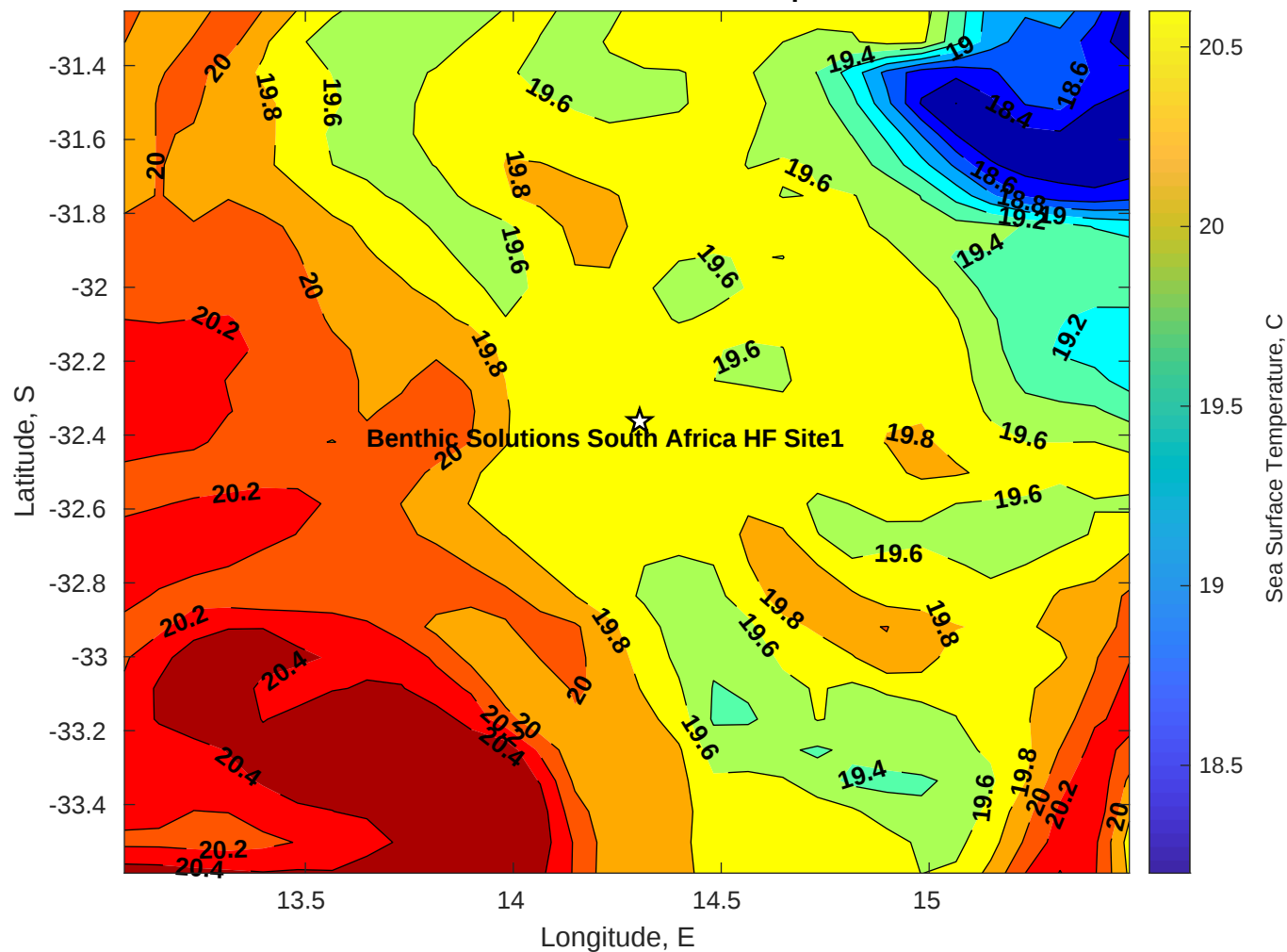
SST for Benthic Solutions South Africa HF Site1 at 18-Apr-2025 00:00:00
