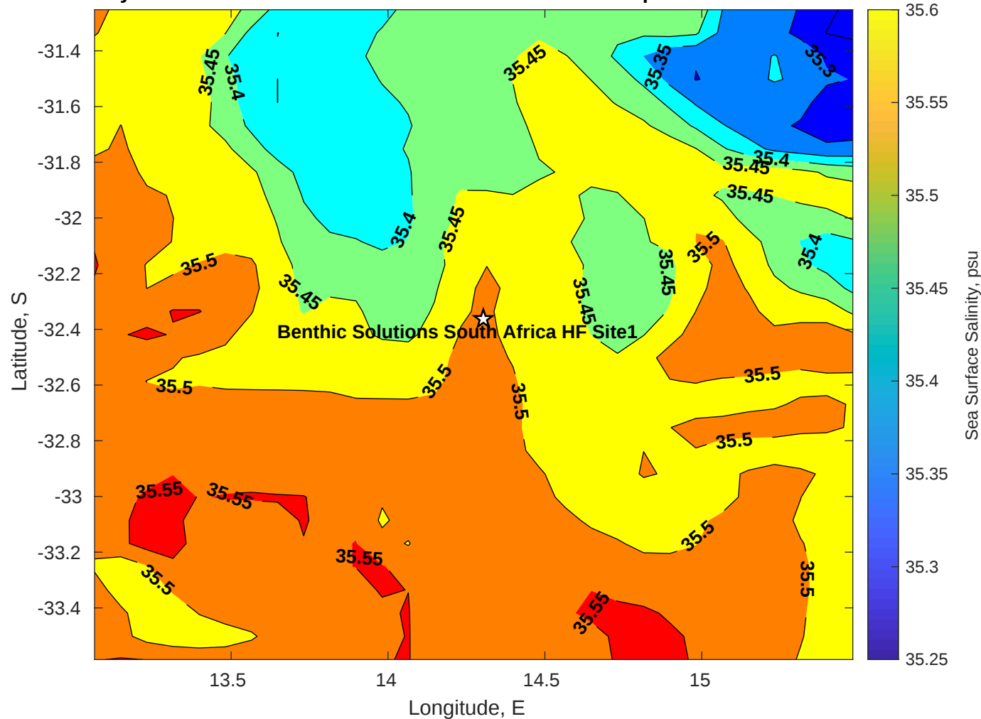
Surface Salinity for Benthic Solutions South Africa HF Site1 at 18-Apr-2025 00:00:00
