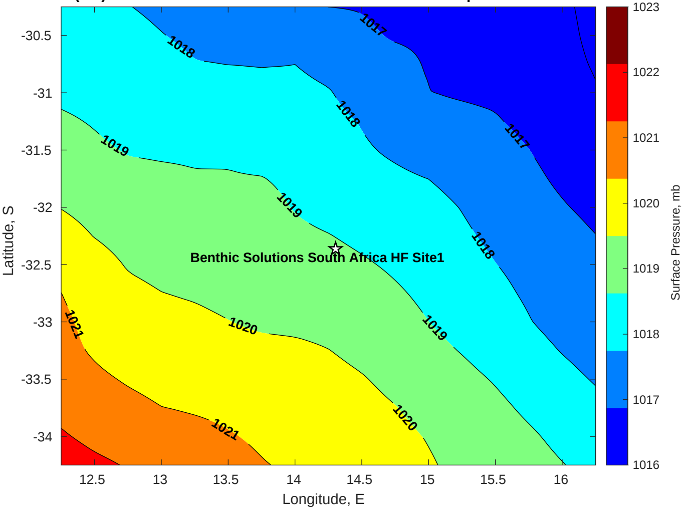
Surface Pressure (mb) for Benthic Solutions South Africa HF Site1 at 20-Apr-2025 00:00:00
