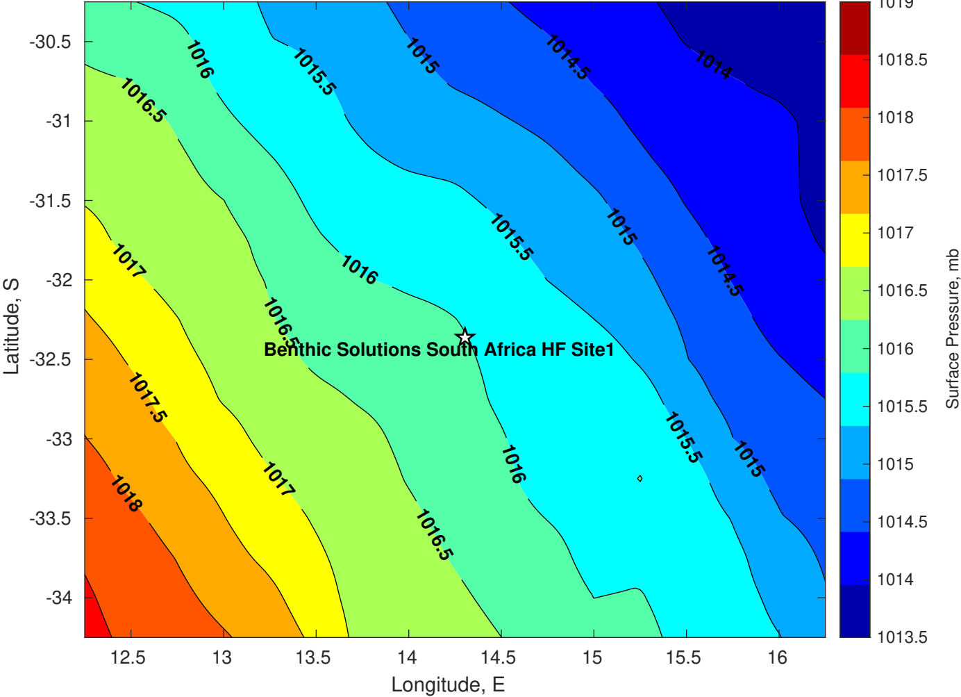
Surface Pressure (mb) for Benthic Solutions South Africa HF Site1 at 19-Apr-2025 00:00:00
