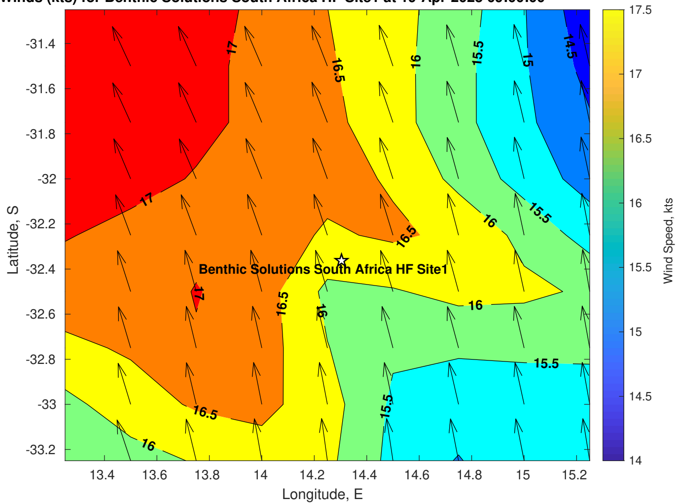
Winds (kts) for Benthic Solutions South Africa HF Site1 at 19-Apr-2025 09:00:00
