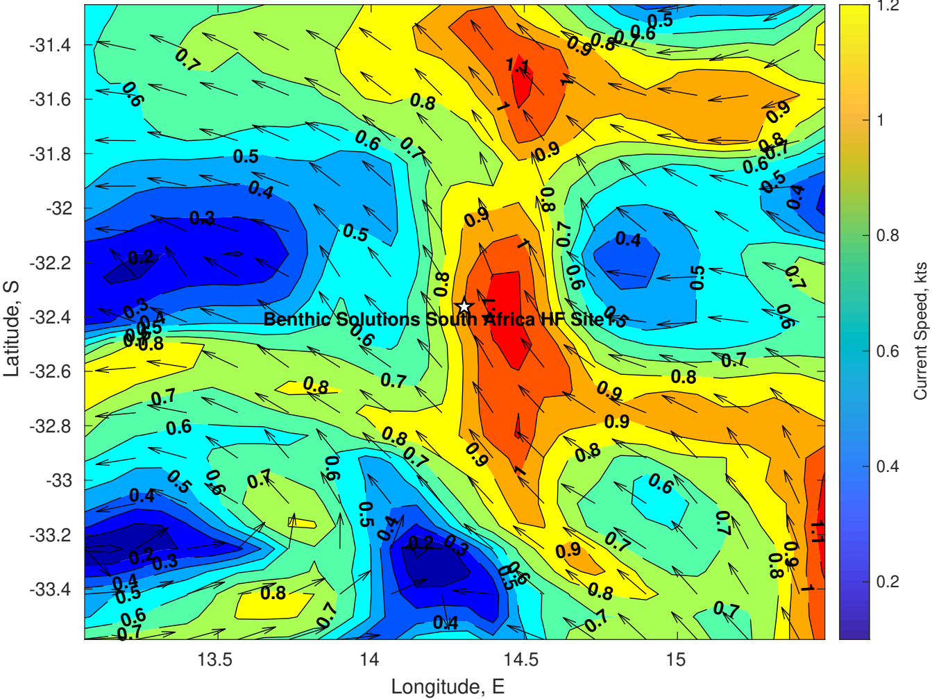
Surface Currents for Benthic Solutions South Africa HF Site1 at 18-Apr-2025 00:00:00
