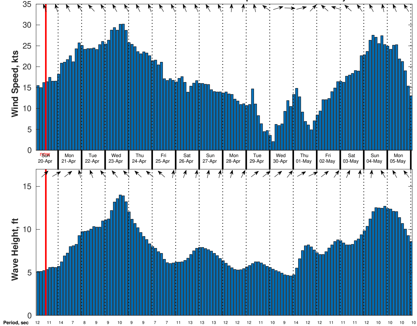
Wind & Wave Forecast for Benthic Solutions South Africa HF Site1 from 19-Apr-2025 02:00:00 to 05-May-2025 02:00:00
