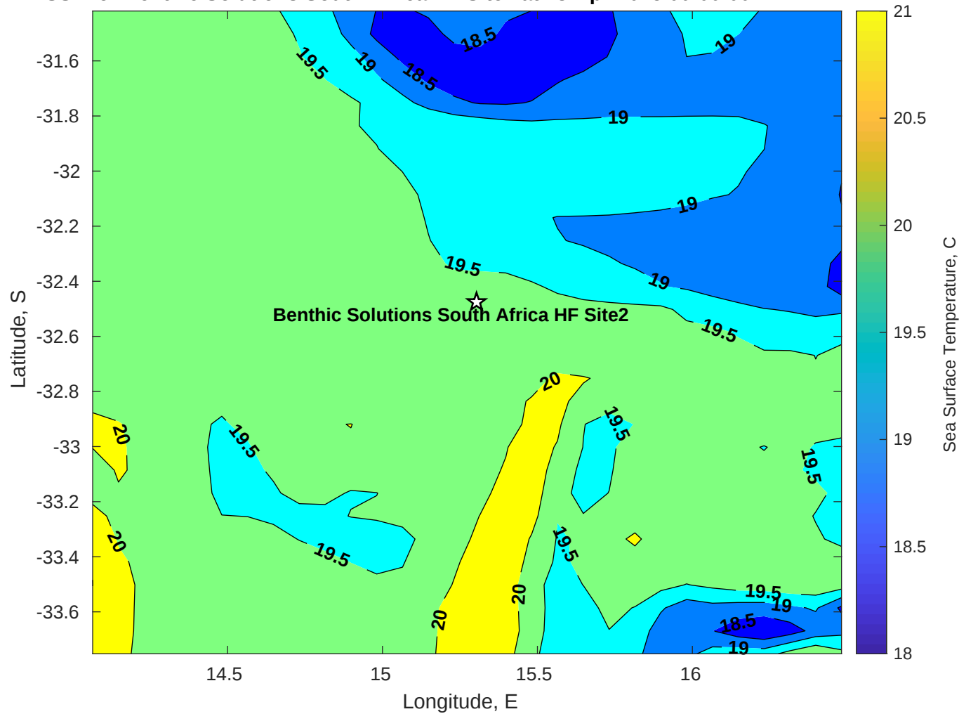
SST for Benthic Solutions South Africa HF Site2 at 18-Apr-2025 00:00:00
