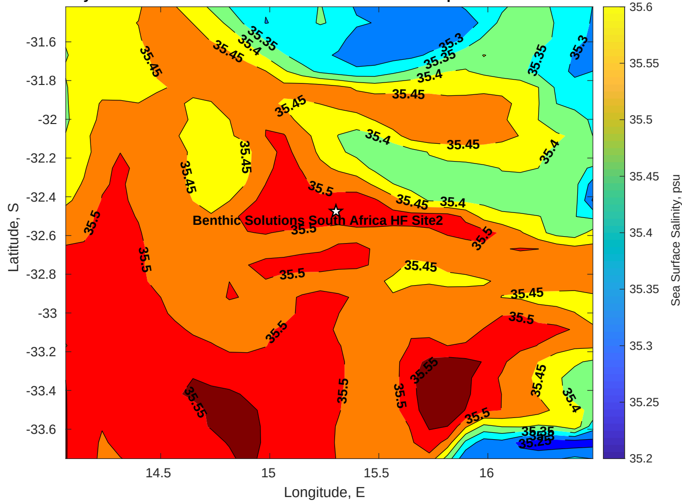
Surface Salinity for Benthic Solutions South Africa HF Site2 at 18-Apr-2025 00:00:00
