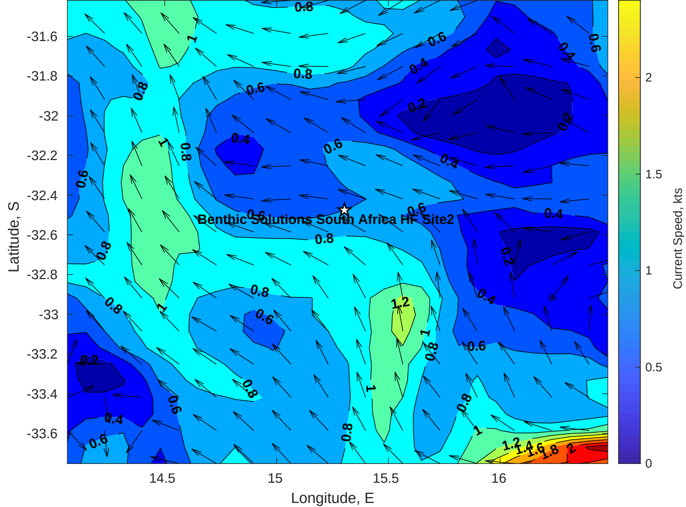
Surface Currents for Benthic Solutions South Africa HF Site2 at 18-Apr-2025 00:00:00
