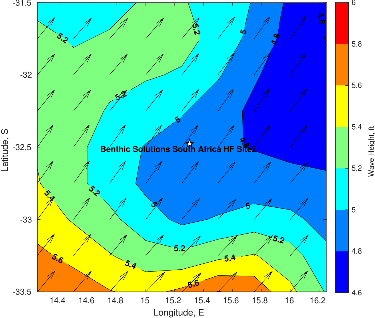
Wave Height (ft) for Benthic Solutions South Africa HF Site2 at 19-Apr-2025 09:00:00
