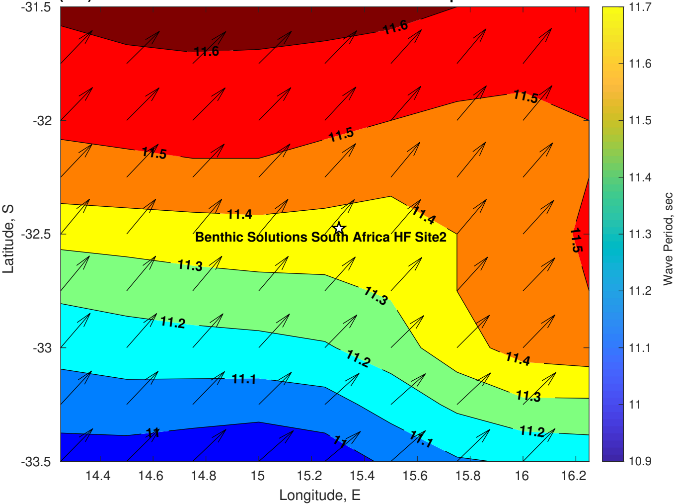
Wave Period (sec) for Benthic Solutions South Africa HF Site2 at 19-Apr-2025 09:00:00
