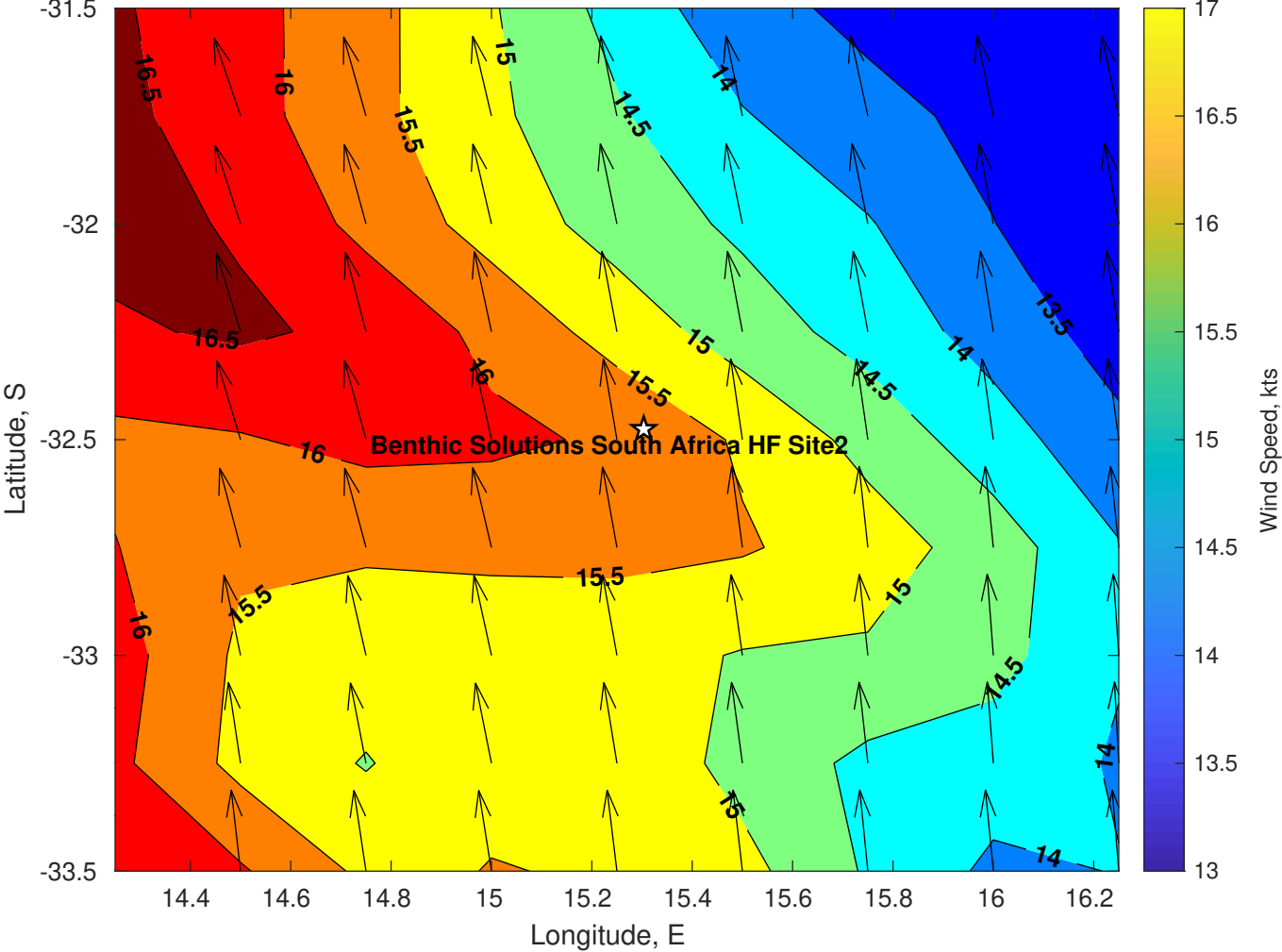
Winds (kts) for Benthic Solutions South Africa HF Site2 at 19-Apr-2025 09:00:00
