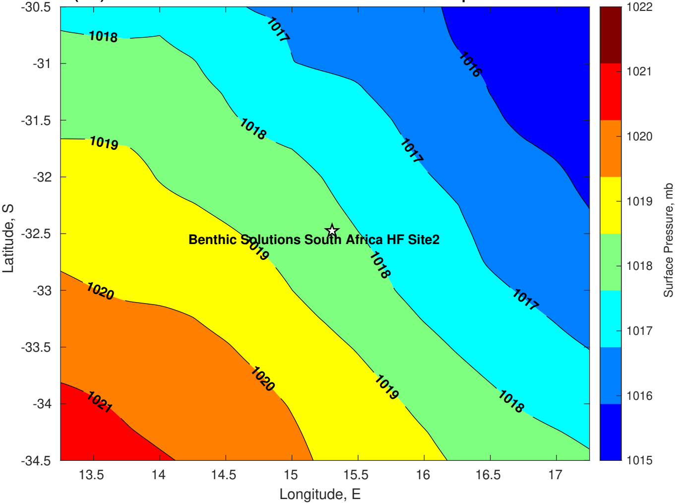
Surface Pressure (mb) for Benthic Solutions South Africa HF Site2 at 20-Apr-2025 00:00:00
