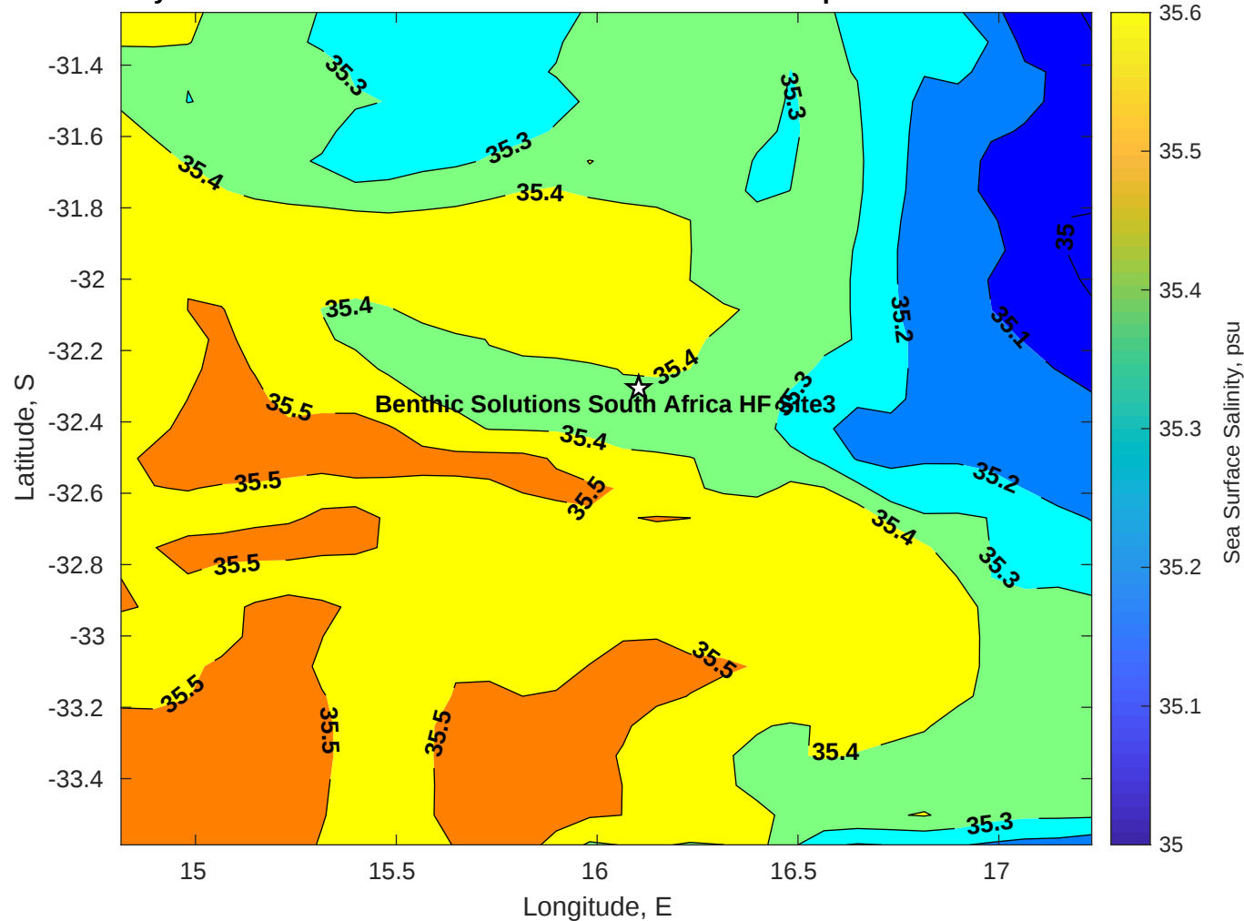
Surface Salinity for Benthic Solutions South Africa HF Site3 at 18-Apr-2025 00:00:00
