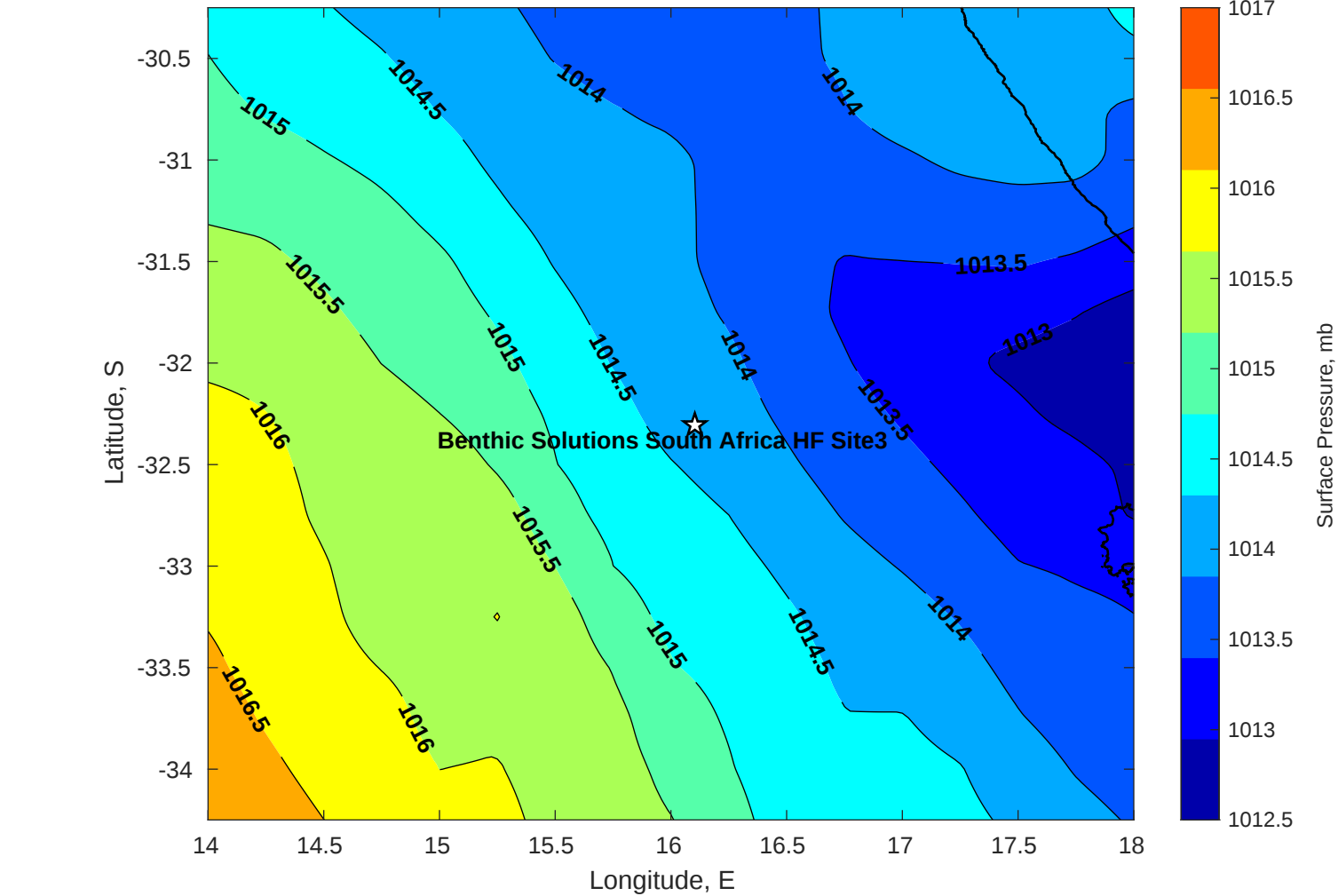
Surface Pressure (mb) for Benthic Solutions South Africa HF Site3 at 19-Apr-2025 00:00:00
