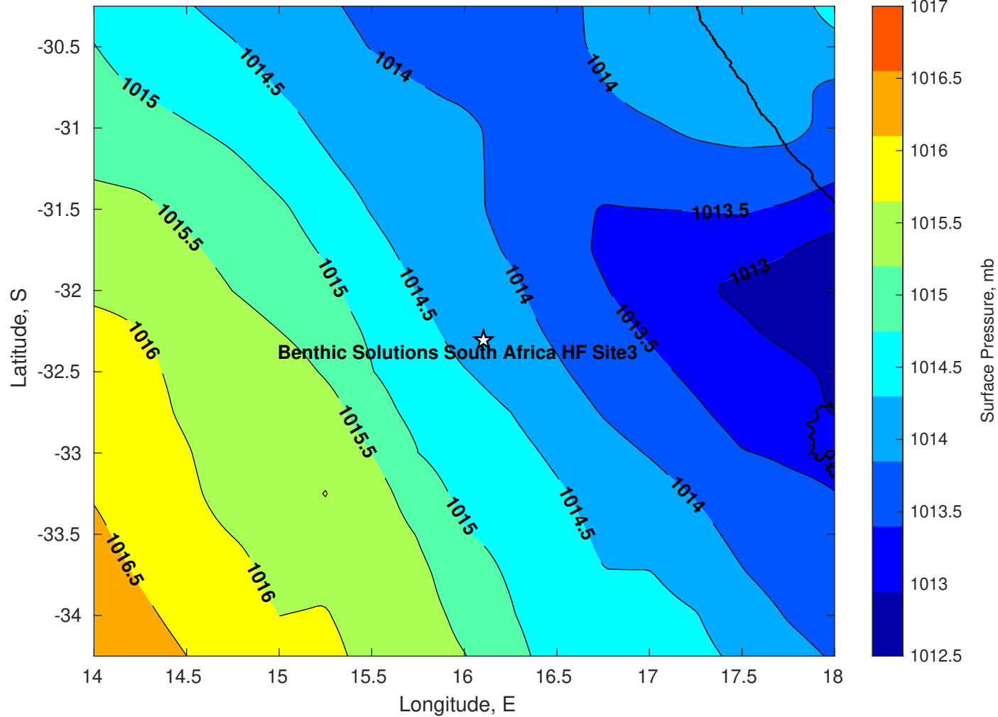
Surface Pressure (mb) for Benthic Solutions South Africa HF Site3 at 19-Apr-2025 00:00:00
