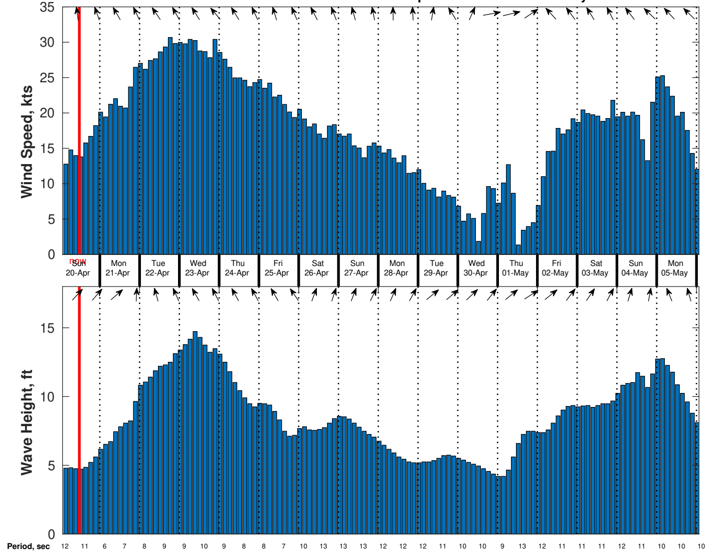
Wind & Wave Forecast for Benthic Solutions South Africa HF Site3 from 19-Apr-2025 02:00:00 to 05-May-2025 02:00:00
