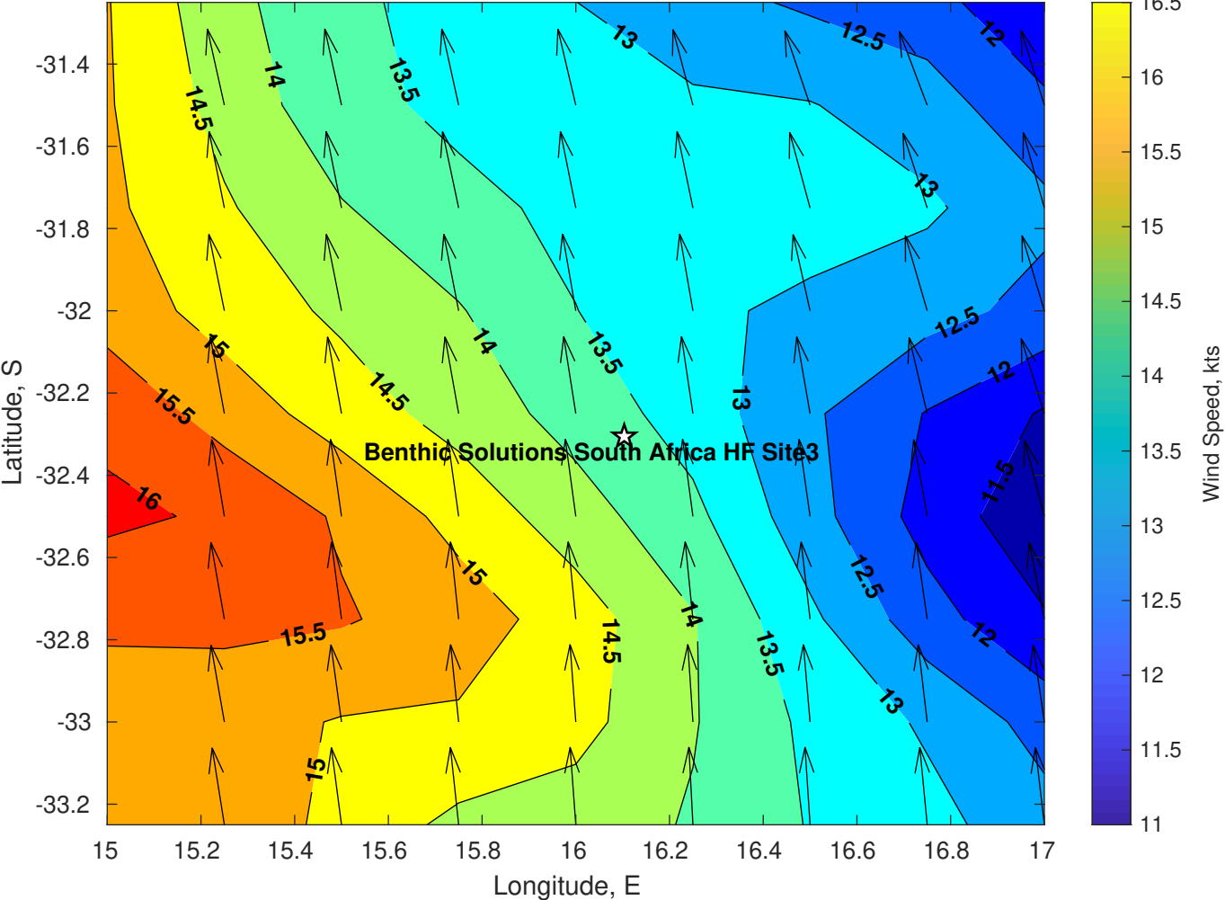
Winds (kts) for Benthic Solutions South Africa HF Site3 at 19-Apr-2025 09:00:00
