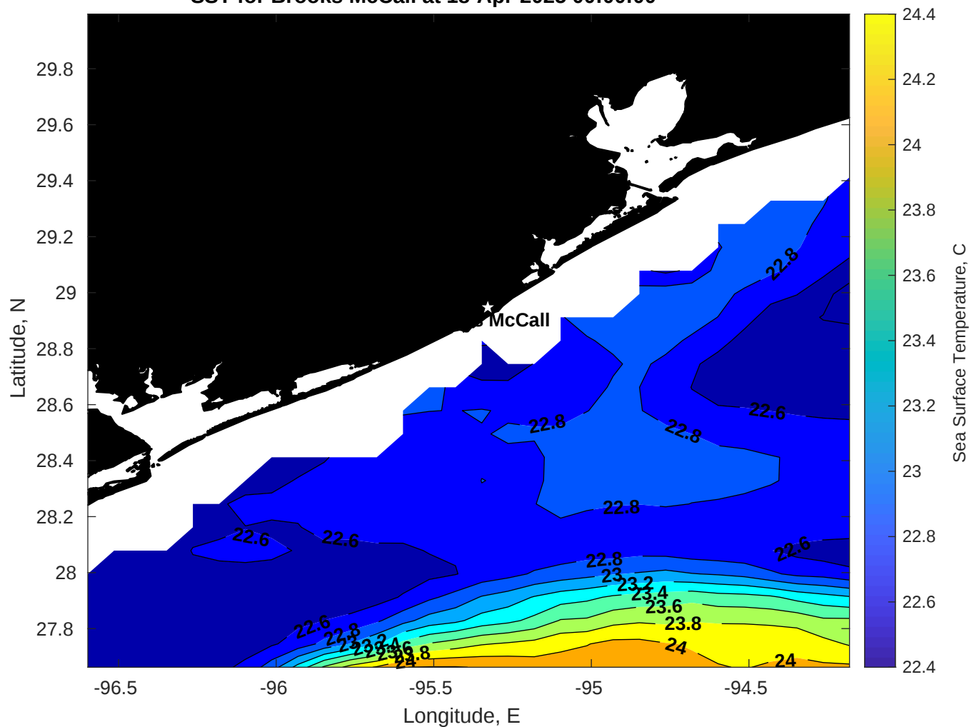
SST for Brooks McCall at 18-Apr-2025 00:00:00
