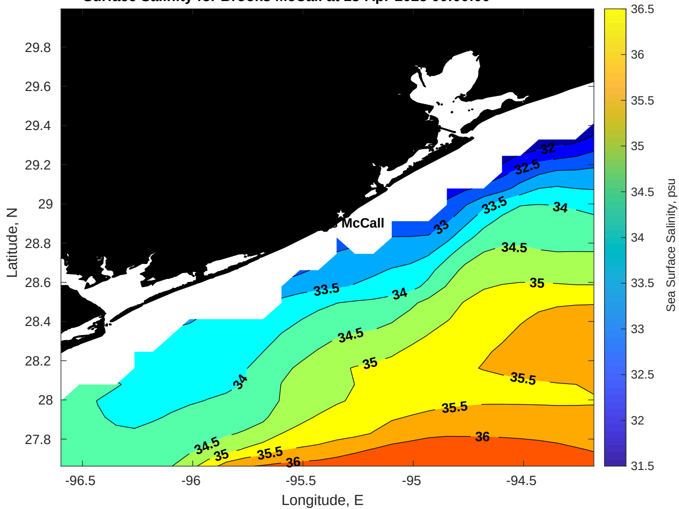
Surface Salinity for Brooks McCall at 18-Apr-2025 00:00:00
