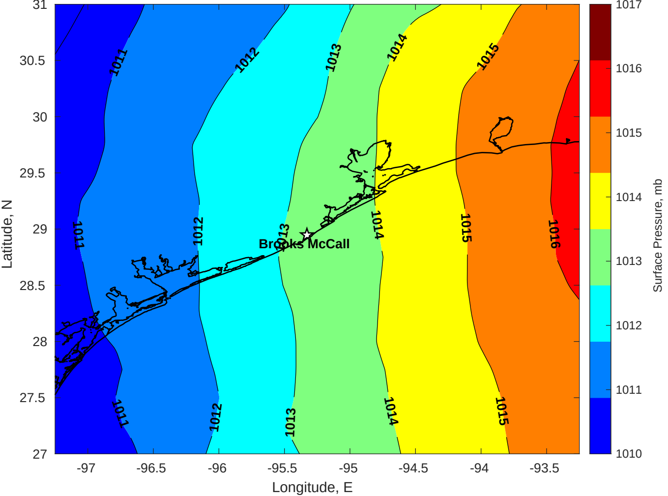
Surface Pressure (mb) for Brooks McCall at 19-Apr-2025 00:00:00
