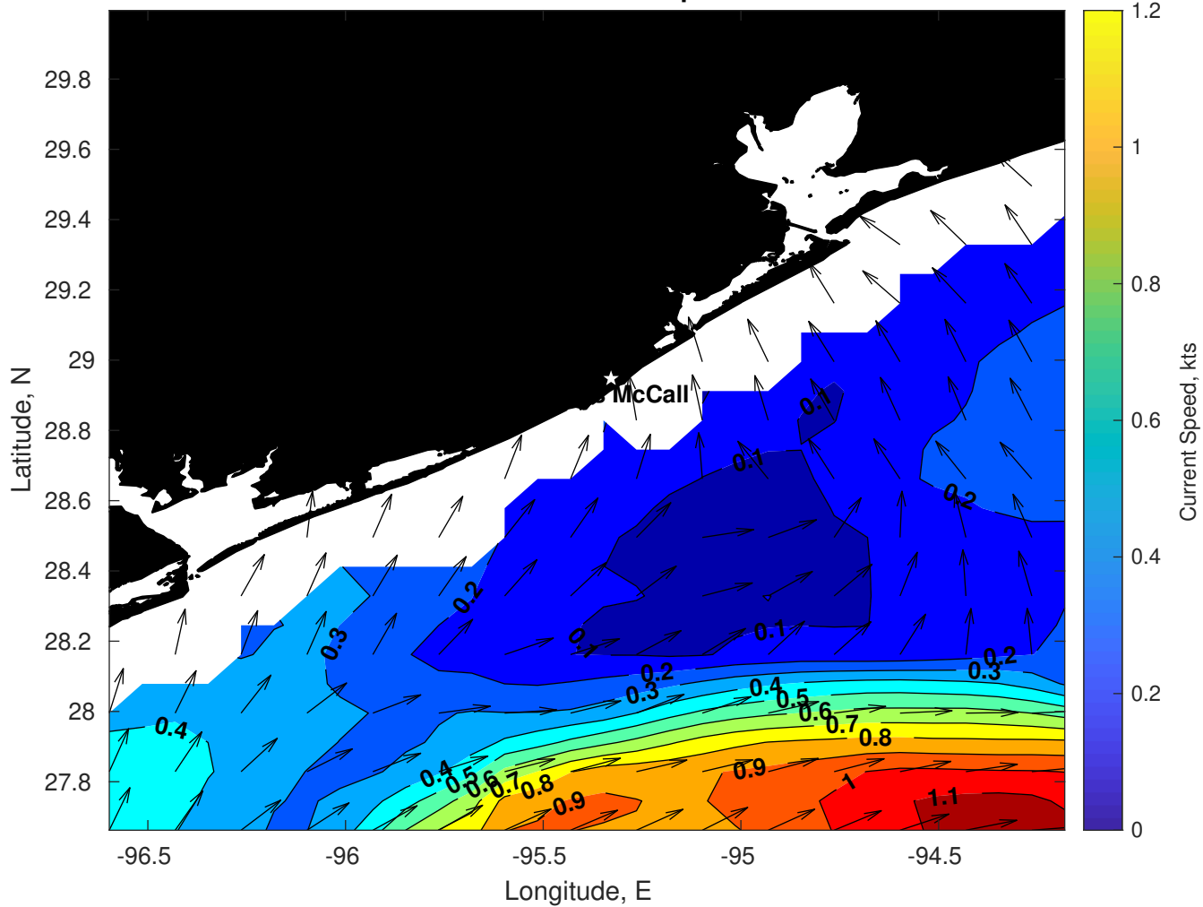
Surface Currents for Brooks McCall at 18-Apr-2025 00:00:00
