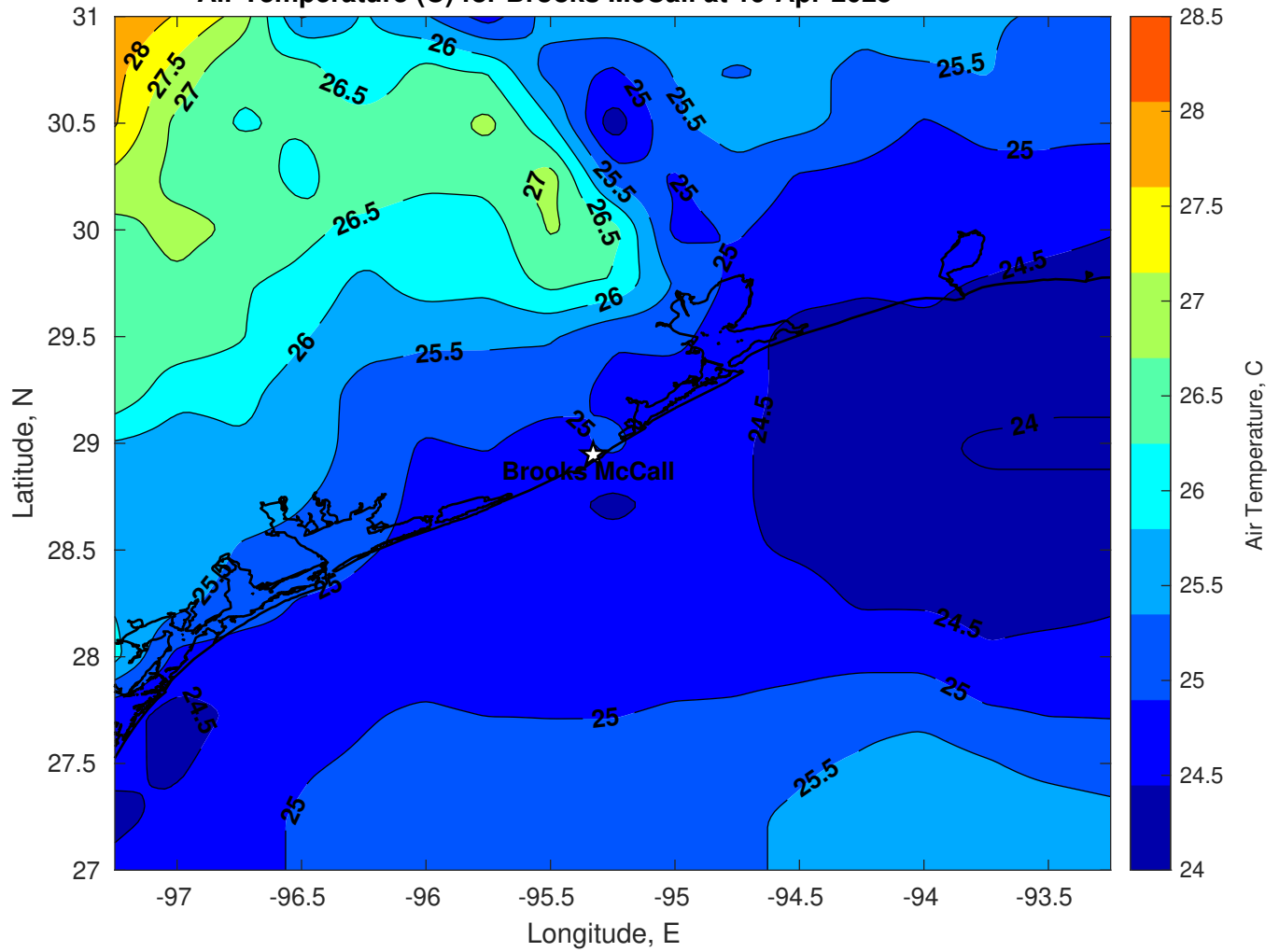
Air Temperature (C) for Brooks McCall at 19-Apr-2025
