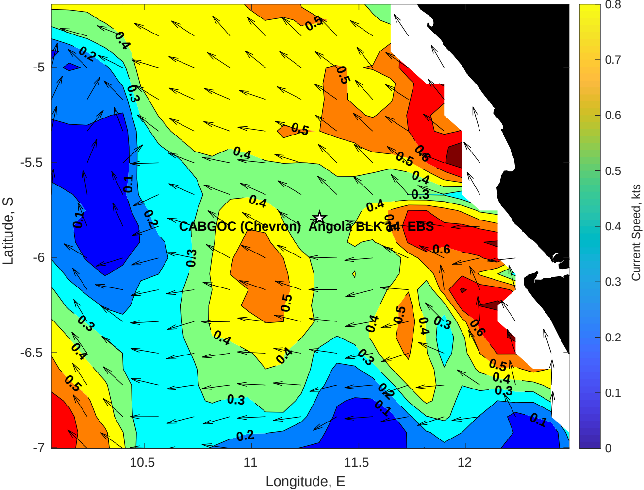
Surface Currents for CABGOC (Chevron) Angola BLK 14 EBS at 18-Apr-2025 00:00:00
