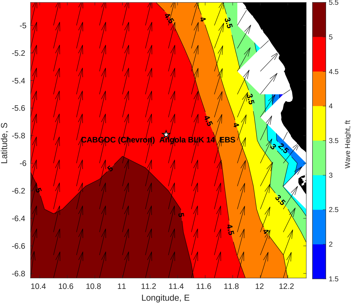
Wave Height (ft) for CABGOC (Chevron) Angola BLK 14 EBS at 19-Apr-2025 09:00:00
