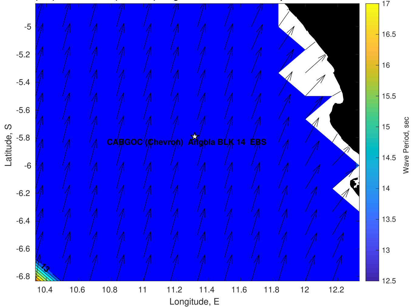
Wave Period (sec) for CABGOC (Chevron) Angola BLK 14 EBS at 19-Apr-2025 09:00:00
