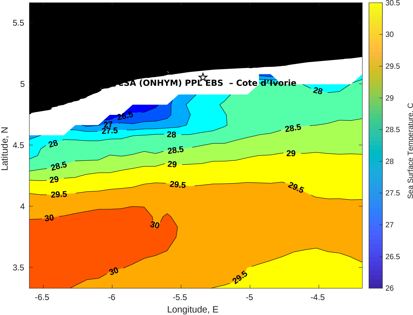
SST for CSA (ONHYM) PPL EBS - Cote d'Ivoire at 18-Apr-2025 00:00:00
