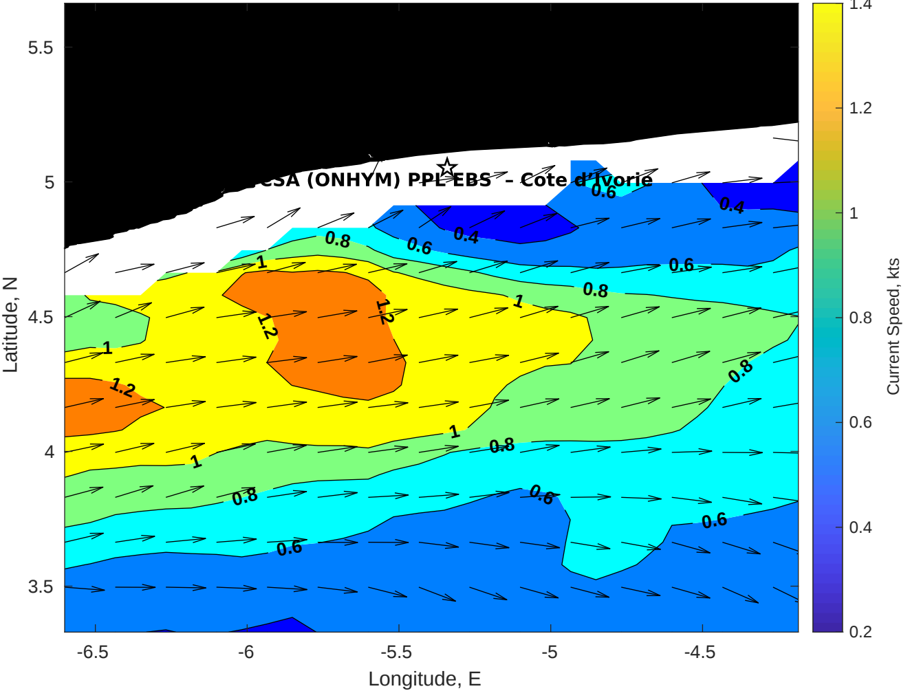
Surface Currents for CSA (ONHYM) PPL EBS - Cote d'Ivoire at 18-Apr-2025 00:00:00
