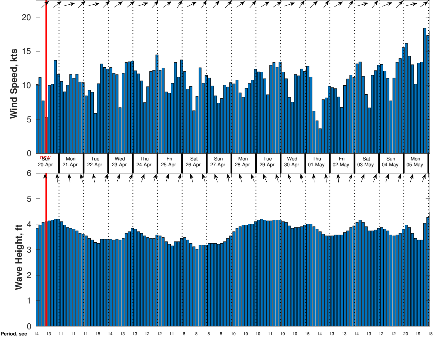
Wind & Wave Forecast for CSA (ONHYM) PPL EBS - Cote d'Ivoire from 19-Apr-2025 01:00:00 to 05-May-2025 01:00:00
