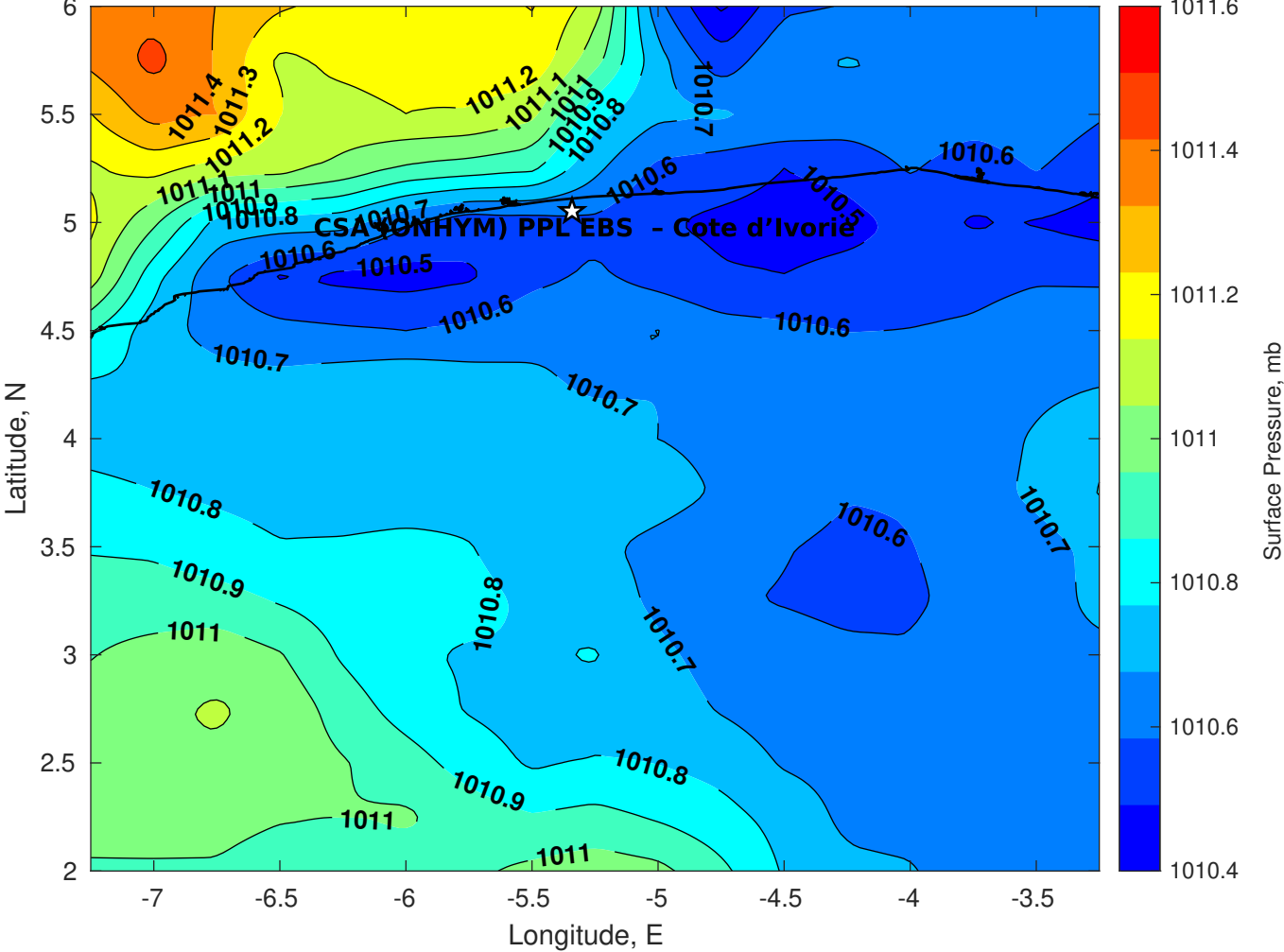
Surface Pressure (mb) for CSA (ONHYM) PPL EBS - Cote d'Ivoire at 19-Apr-2025 00:00:00
