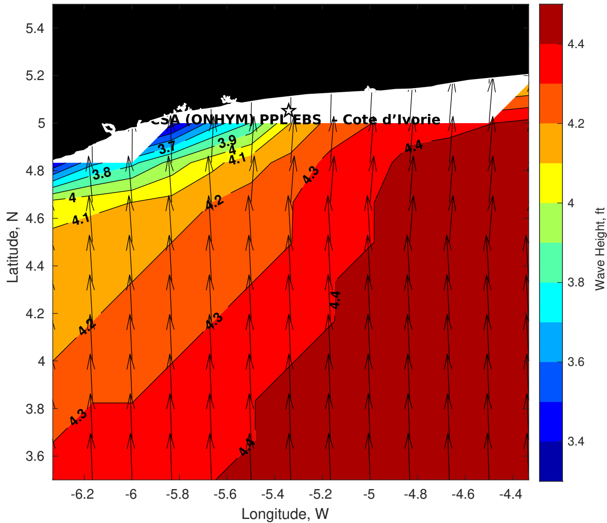
Wave Height (ft) for CSA (ONHYM) PPL EBS - Cote d'Ivoire at 19-Apr-2025 09:00:00
