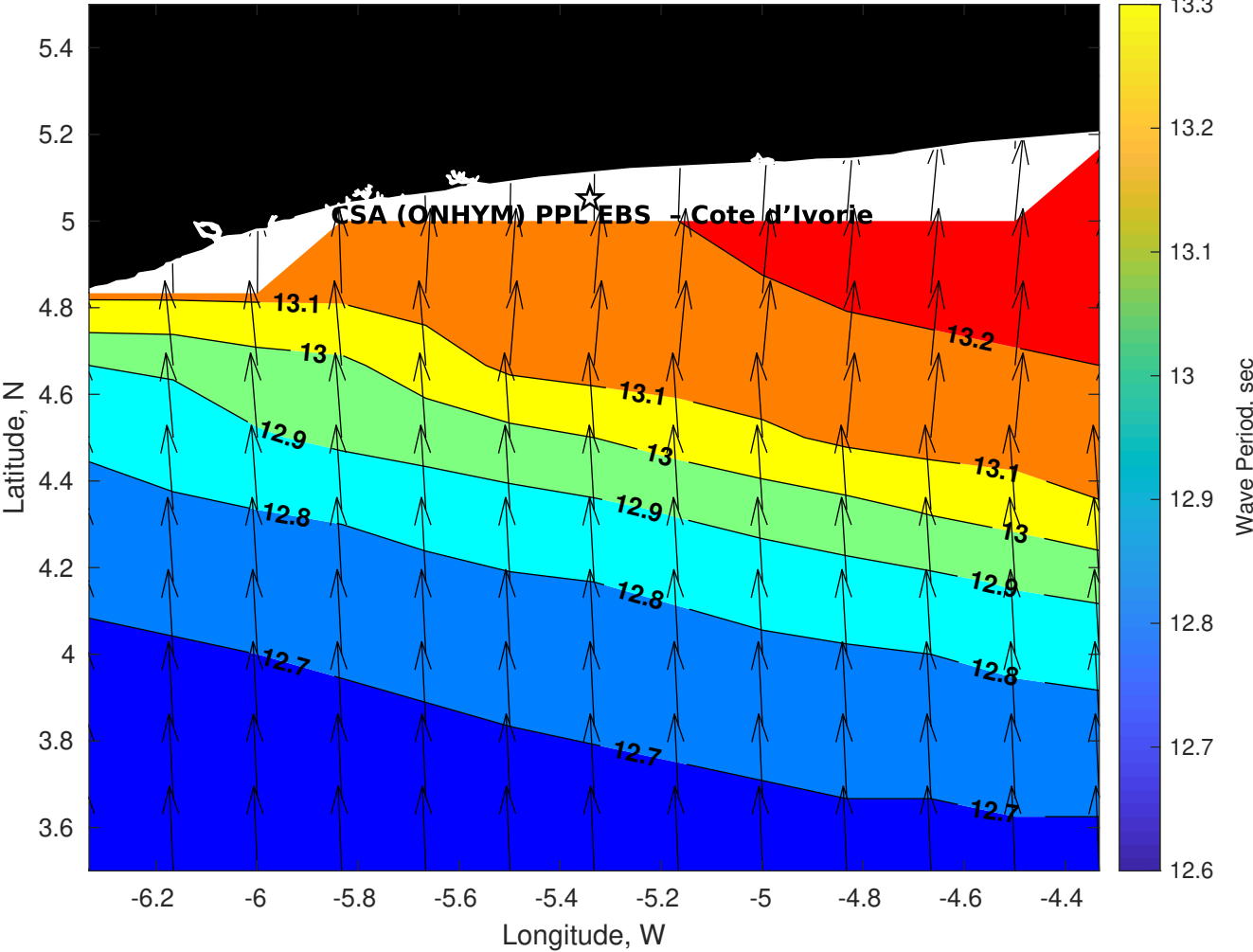
Wave Period (sec) for CSA (ONHYM) PPL EBS - Cote d'Ivoire at 19-Apr-2025 09:00:00
