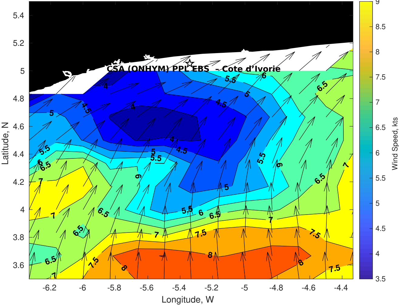
Winds (kts) for CSA (ONHYM) PPL EBS - Cote d'Ivoire at 19-Apr-2025 09:00:00
