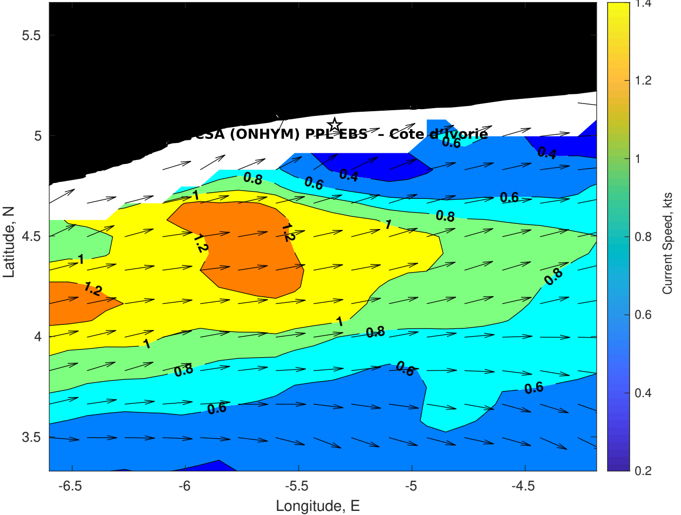
Surface Currents for CSA (ONHYM) PPL EBS - Cote d'Ivoire at 18-Apr-2025 00:00:00
