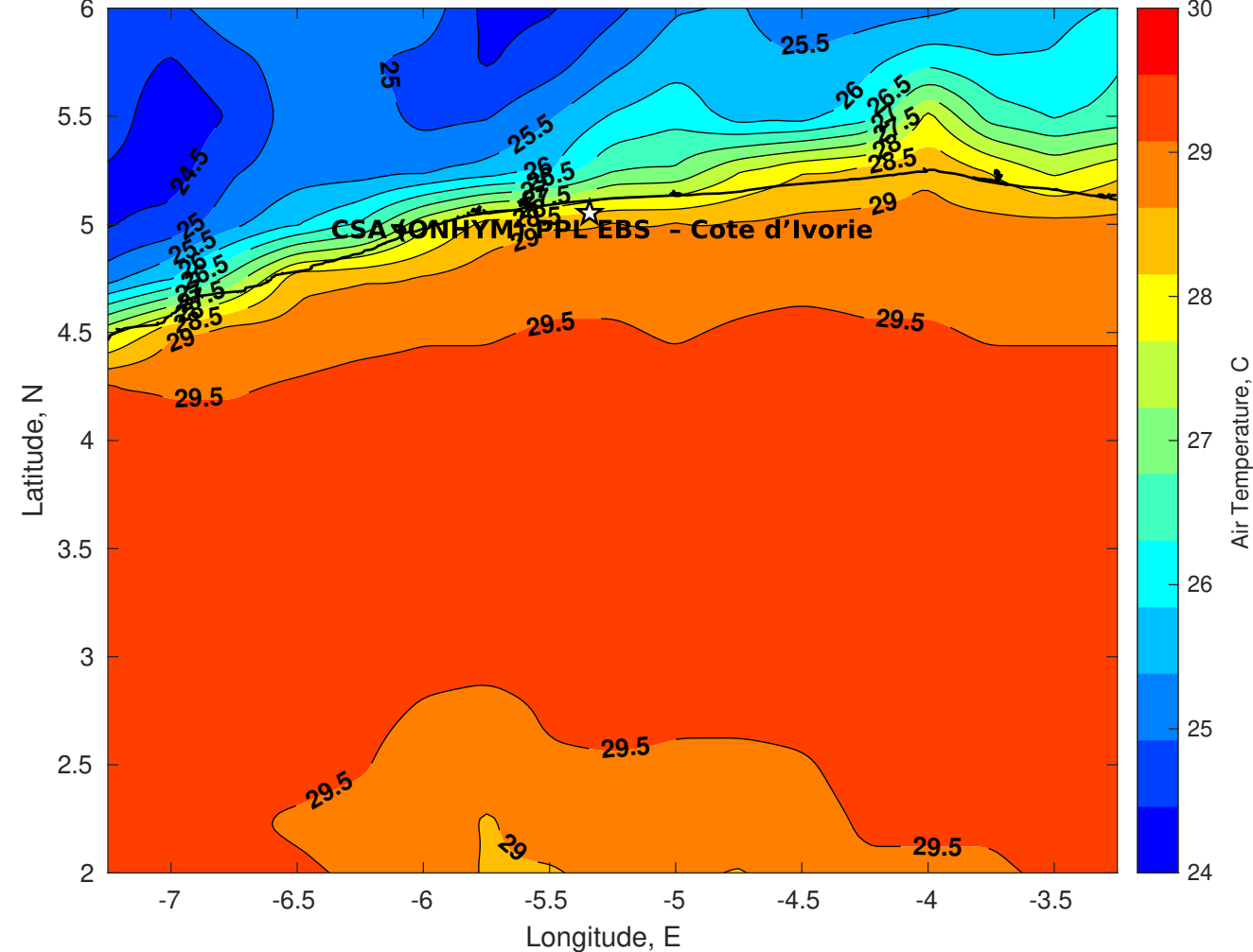
Air Temperature (C) for CSA (ONHYM) PPL EBS - Cote d'Ivoire at 19-Apr-2025
