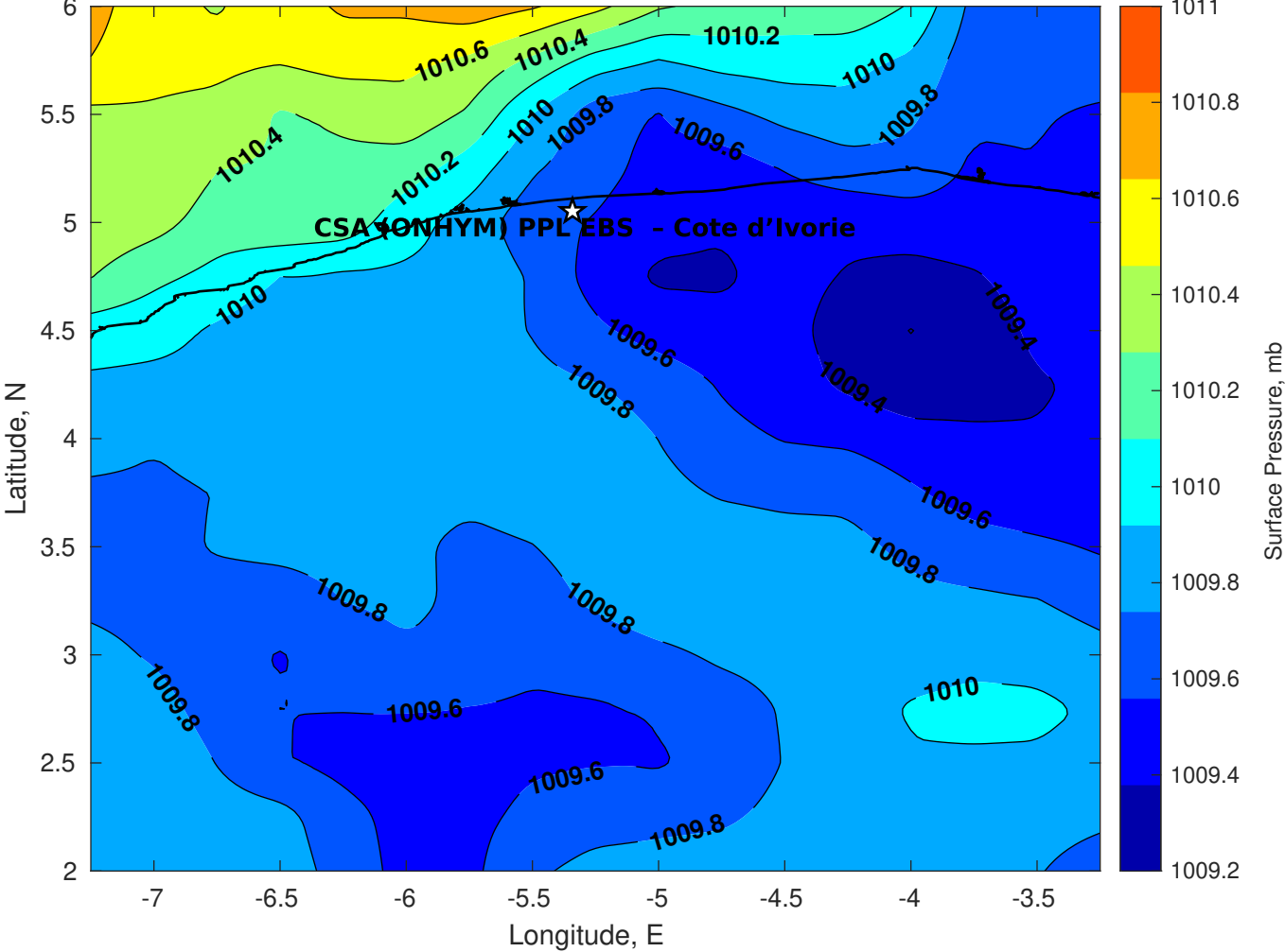
Surface Pressure (mb) for CSA (ONHYM) PPL EBS - Cote d'Ivoire at 20-Apr-2025 00:00:00
