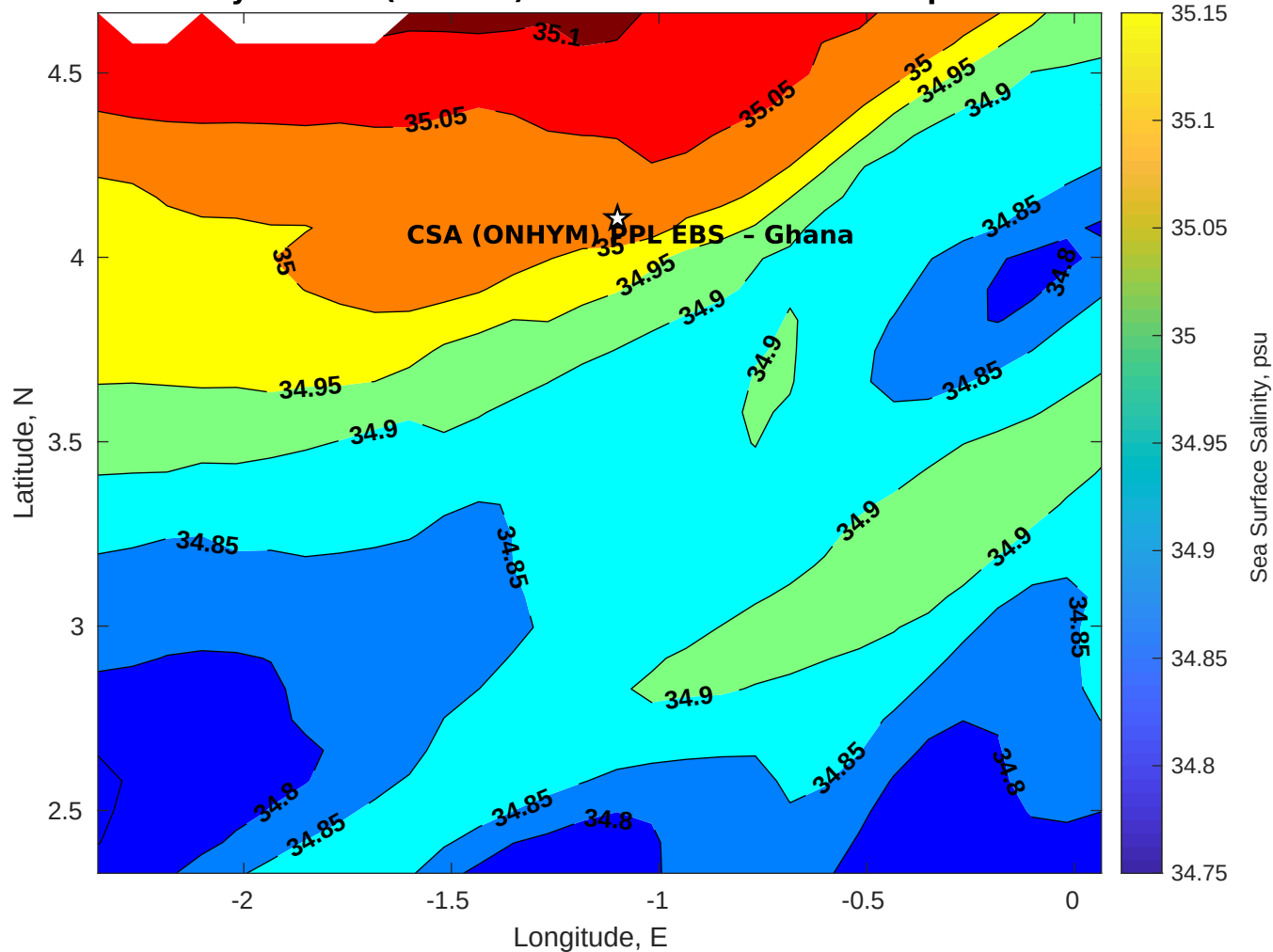
Surface Salinity for CSA (ONHYM) PPL EBS - Ghana at 18-Apr-2025 00:00:00
