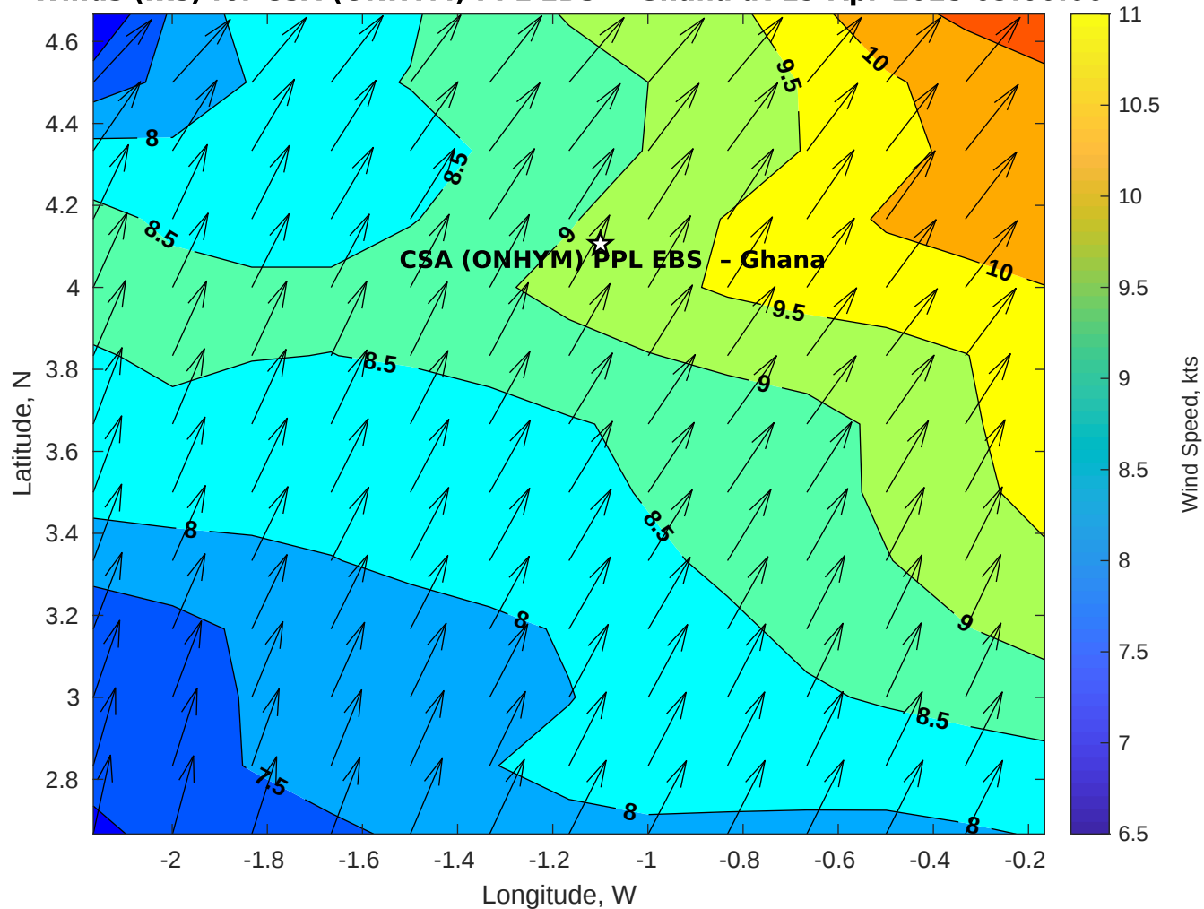
Winds (kts) for CSA (ONHYM) PPL EBS - Ghana at 19-Apr-2025 09:00:00
