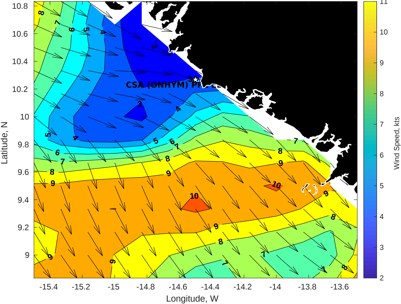
Winds (kts) for CSA (ONHYM) PPL EBS - Guinea at 19-Apr-2025 09:00:00
