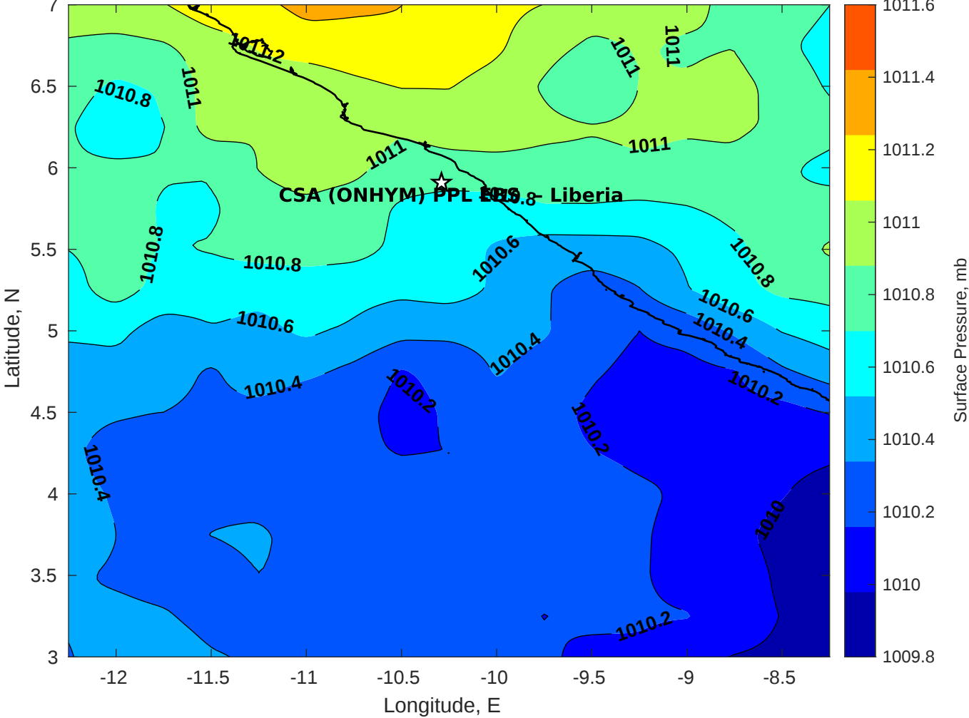
Surface Pressure (mb) for CSA (ONHYM) PPL EBS - Liberia at 20-Apr-2025 00:00:00
