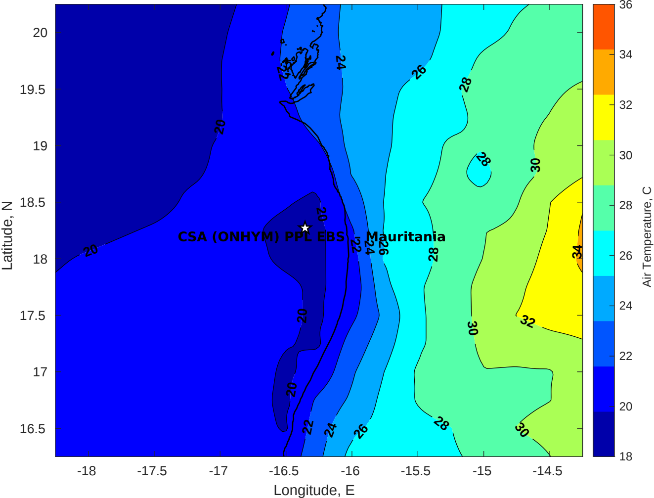
Air Temperature (C) for CSA (ONHYM) PPL EBS - Mauritania at 19-Apr-2025
